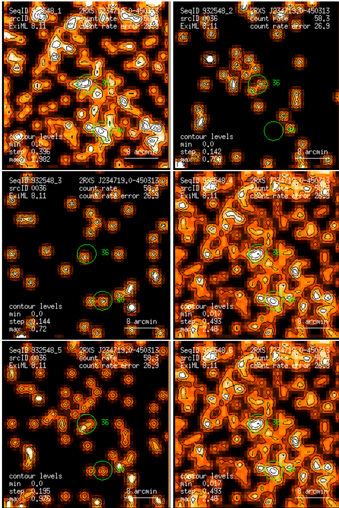
Figure 36: RASS 932548: detection 0036: band rate images, Gaussian filter: (1) PSPC channels 11 – 41, (2) 52 – 90, (3) 91 – 201, (4) 11 – 235, (5) 52 – 201, (6) 11 – 201. Broad band rates in counts/ks. Band rate contour levels in counts/ks/arcmin 2 .
