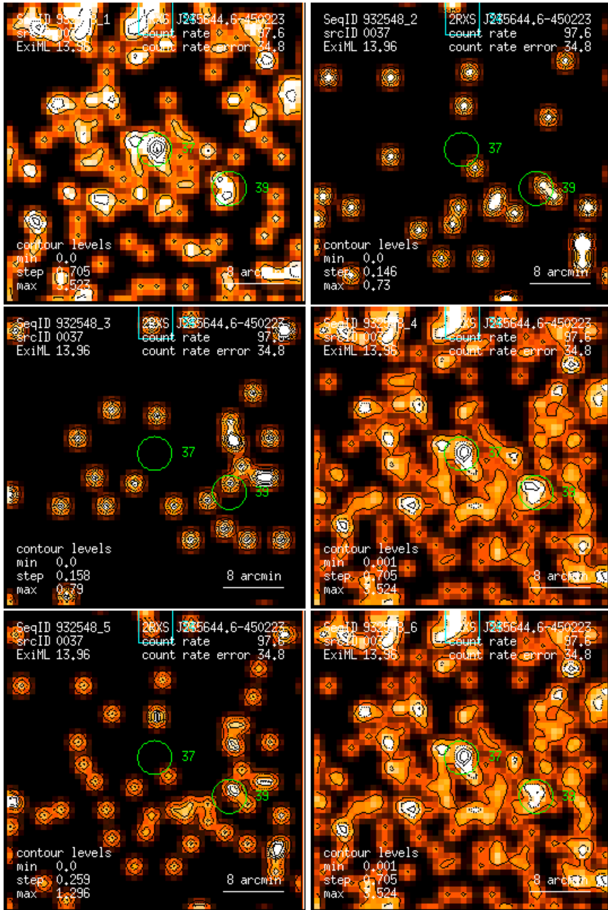
Figure 37: RASS 932548: detection 0037: band rate images, Gaussian filter: (1) PSPC channels 11 – 41, (2) 52 – 90, (3) 91 – 201, (4) 11 – 235, (5) 52 – 201, (6) 11 – 201. Broad band rates in counts/ks. Band rate contour levels in counts/ks/arcmin 2 .
