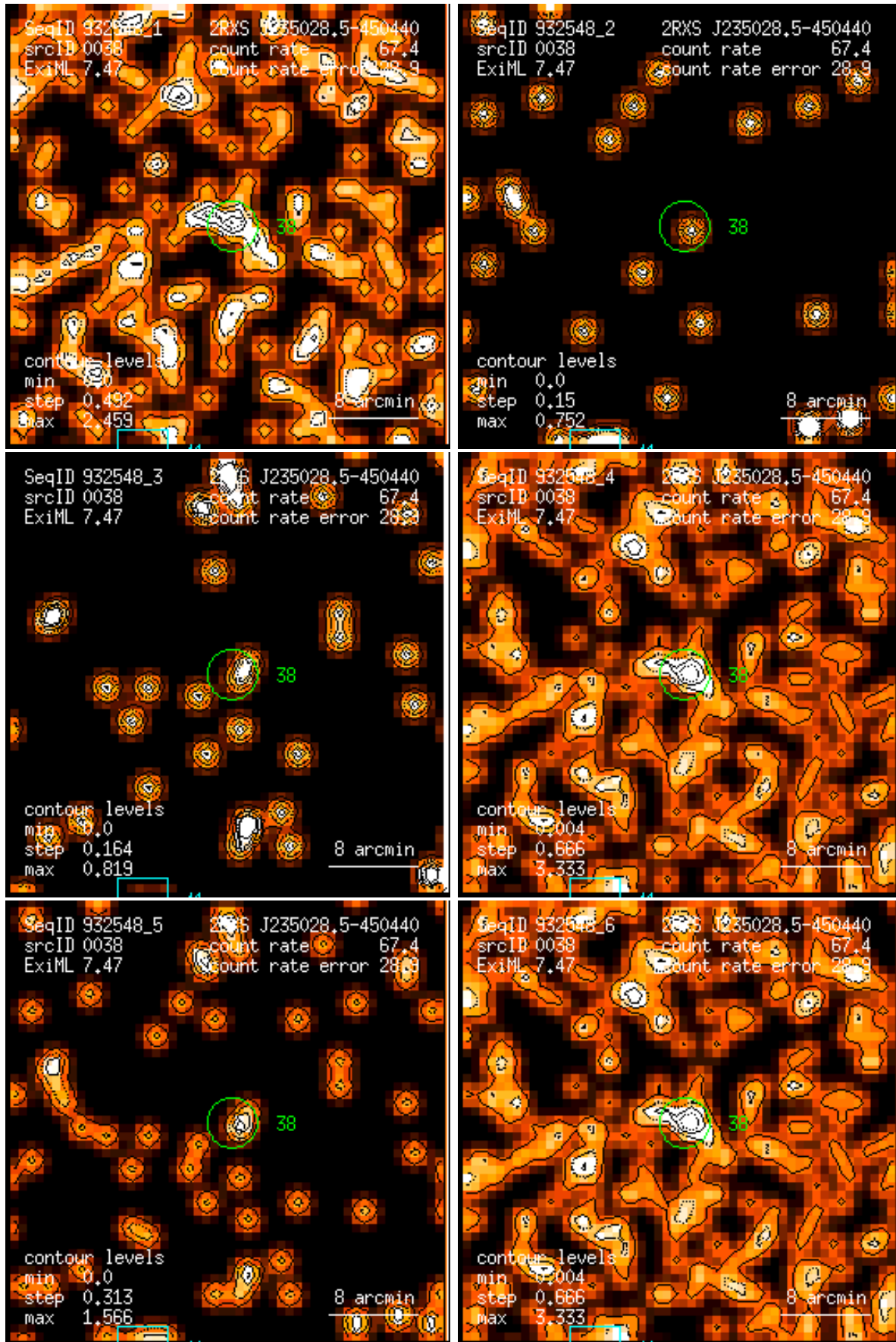
Figure 38: RASS 932548: detection 0038: band rate images, Gaussian filter: (1) PSPC channels 11 – 41, (2) 52 – 90, (3) 91 – 201, (4) 11 – 235, (5) 52 – 201, (6) 11 – 201. Broad band rates in counts/ks. Band rate contour levels in counts/ks/arcmin 2 .
