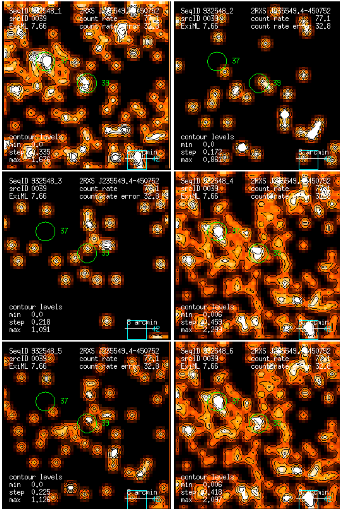
Figure 39: RASS 932548: detection 0039: band rate images, Gaussian filter: (1) PSPC channels 11 – 41, (2) 52 – 90, (3) 91 – 201, (4) 11 – 235, (5) 52 – 201, (6) 11 – 201. Broad band rates in counts/ks. Band rate contour levels in counts/ks/arcmin 2 .
