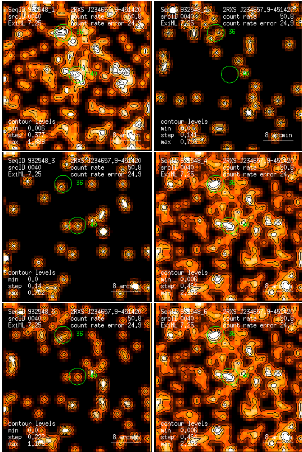
Figure 40: RASS 932548: detection 0040: band rate images, Gaussian filter: (1) PSPC channels 11 – 41, (2) 52 – 90, (3) 91 – 201, (4) 11 – 235, (5) 52 – 201, (6) 11 – 201. Broad band rates in counts/ks. Band rate contour levels in counts/ks/arcmin 2 .
