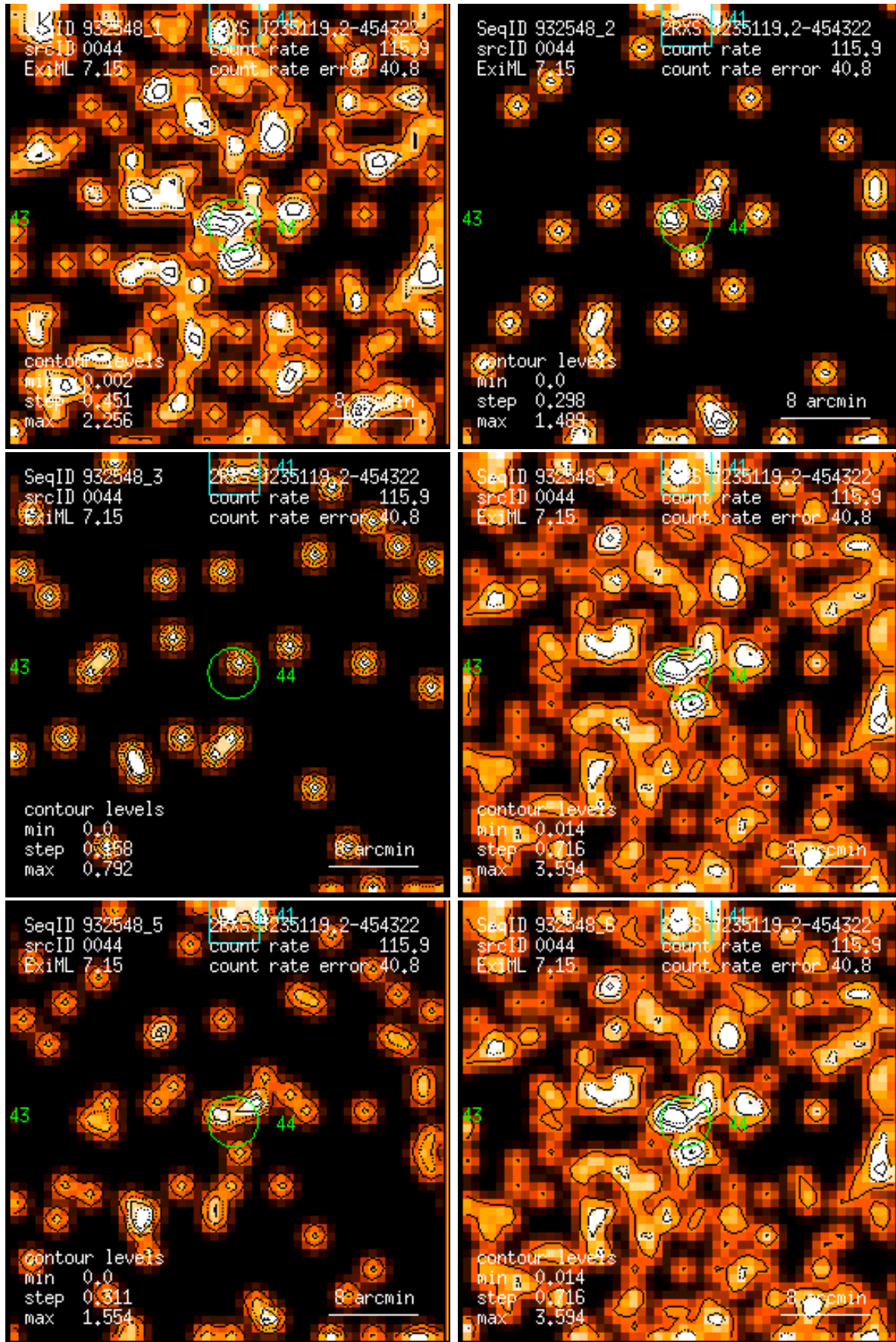
Figure 44: RASS 932548: detection 0044: band rate images, Gaussian filter: (1) PSPC channels 11 – 41, (2) 52 – 90, (3) 91 – 201, (4) 11 – 235, (5) 52 – 201, (6) 11 – 201. Broad band rates in counts/ks. Band rate contour levels in counts/ks/arcmin 2 .
