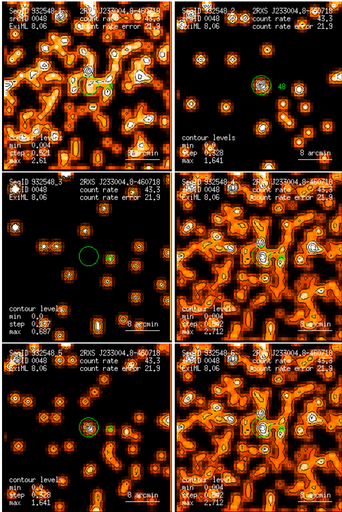
Figure 48: RASS 932548: detection 0048: band rate images, Gaussian filter: (1) PSPC channels 11 – 41, (2) 52 – 90, (3) 91 – 201, (4) 11 – 235, (5) 52 – 201, (6) 11 – 201. Broad band rates in counts/ks. Band rate contour levels in counts/ks/arcmin 2 .
