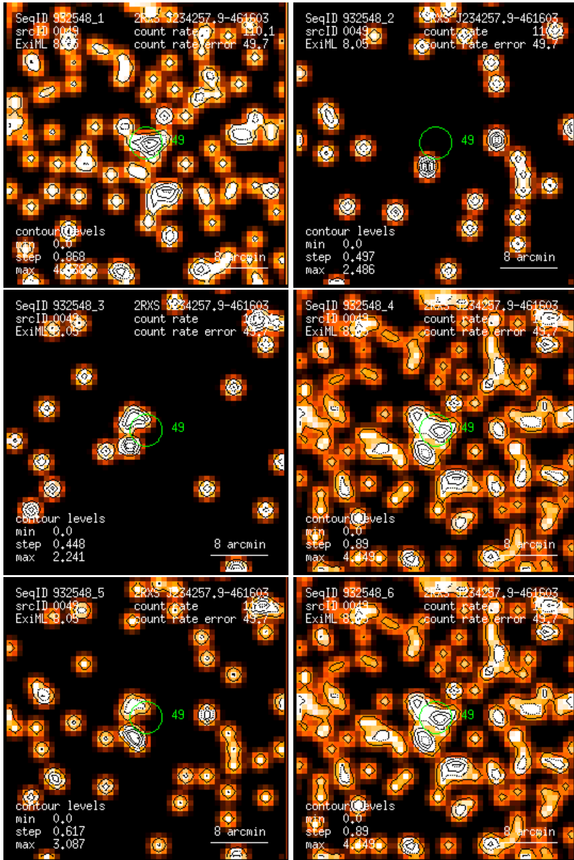
Figure 49: RASS 932548: detection 0049: band rate images, Gaussian filter: (1) PSPC channels 11 – 41, (2) 52 – 90, (3) 91 – 201, (4) 11 – 235, (5) 52 – 201, (6) 11 – 201. Broad band rates in counts/ks. Band rate contour levels in counts/ks/arcmin 2 .
