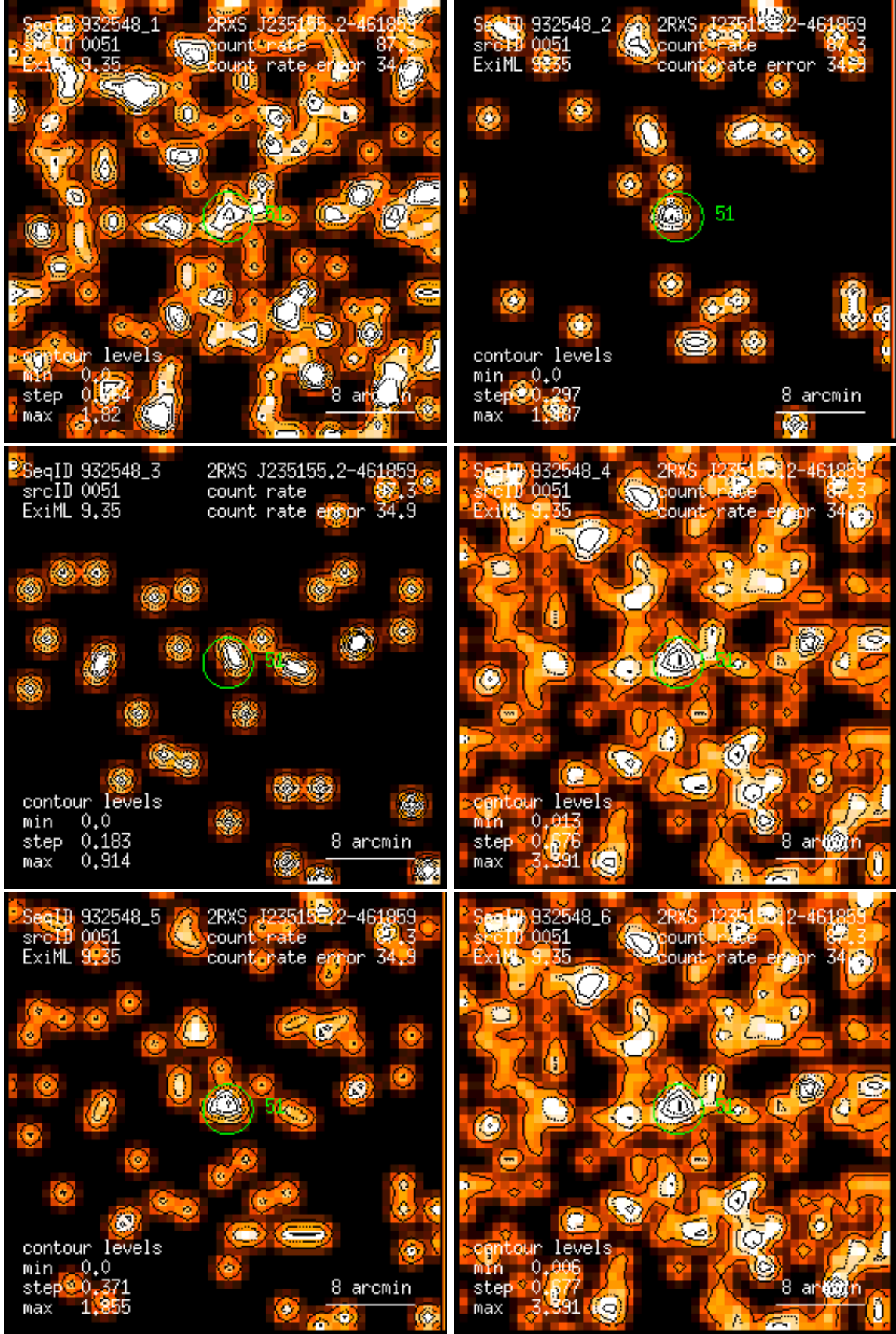
Figure 51: RASS 932548: detection 0051: band rate images, Gaussian filter: (1) PSPC channels 11 – 41, (2) 52 – 90, (3) 91 – 201, (4) 11 – 235, (5) 52 – 201, (6) 11 – 201. Broad band rates in counts/ks. Band rate contour levels in counts/ks/arcmin 2 .
