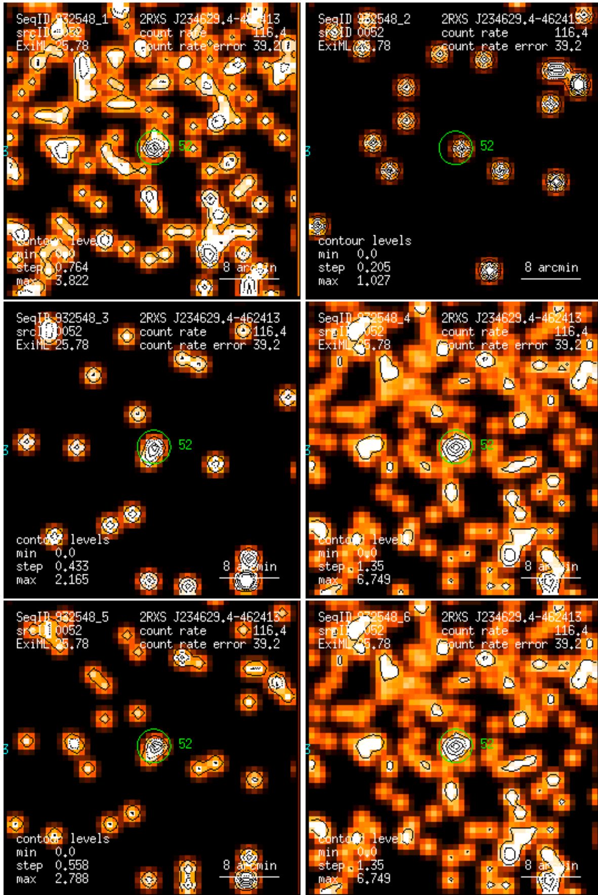
Figure 52: RASS 932548: detection 0052: band rate images, Gaussian filter: (1) PSPC channels 11 – 41, (2) 52 – 90, (3) 91 – 201, (4) 11 – 235, (5) 52 – 201, (6) 11 – 201. Broad band rates in counts/ks. Band rate contour levels in counts/ks/arcmin 2 .
