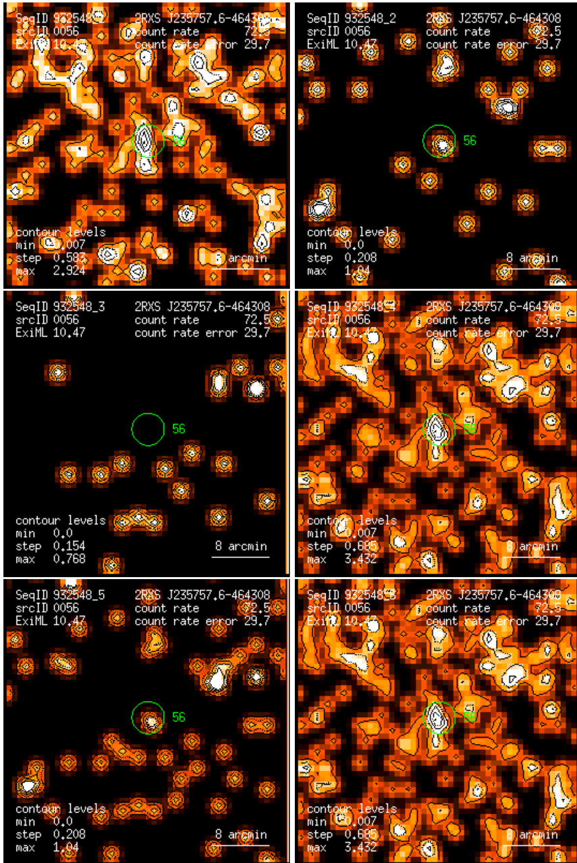
Figure 56: RASS 932548: detection 0056: band rate images, Gaussian filter: (1) PSPC channels 11 – 41, (2) 52 – 90, (3) 91 – 201, (4) 11 – 235, (5) 52 – 201, (6) 11 – 201. Broad band rates in counts/ks. Band rate contour levels in counts/ks/arcmin 2 .
