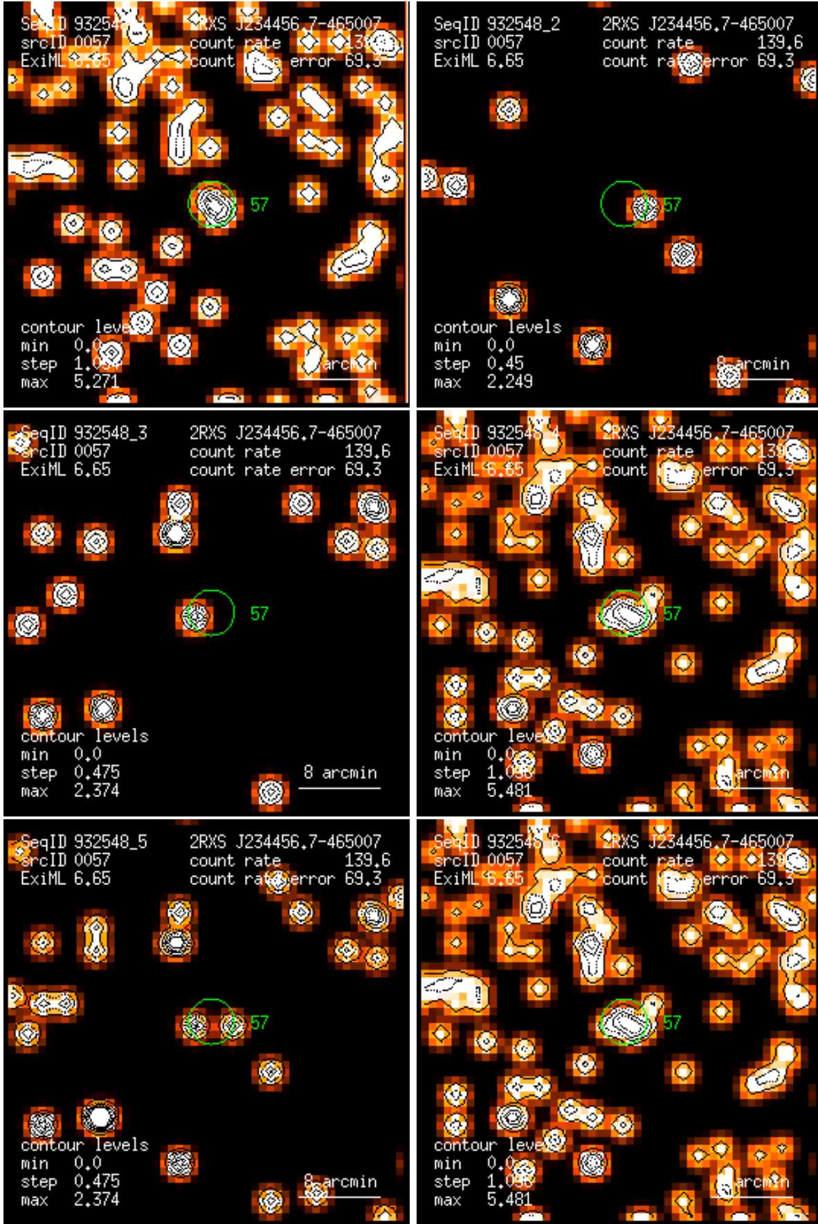
Figure 57: RASS 932548: detection 0057: band rate images, Gaussian filter: (1) PSPC channels 11 – 41, (2) 52 – 90, (3) 91 – 201, (4) 11 – 235, (5) 52 – 201, (6) 11 – 201. Broad band rates in counts/ks. Band rate contour levels in counts/ks/arcmin 2 .
