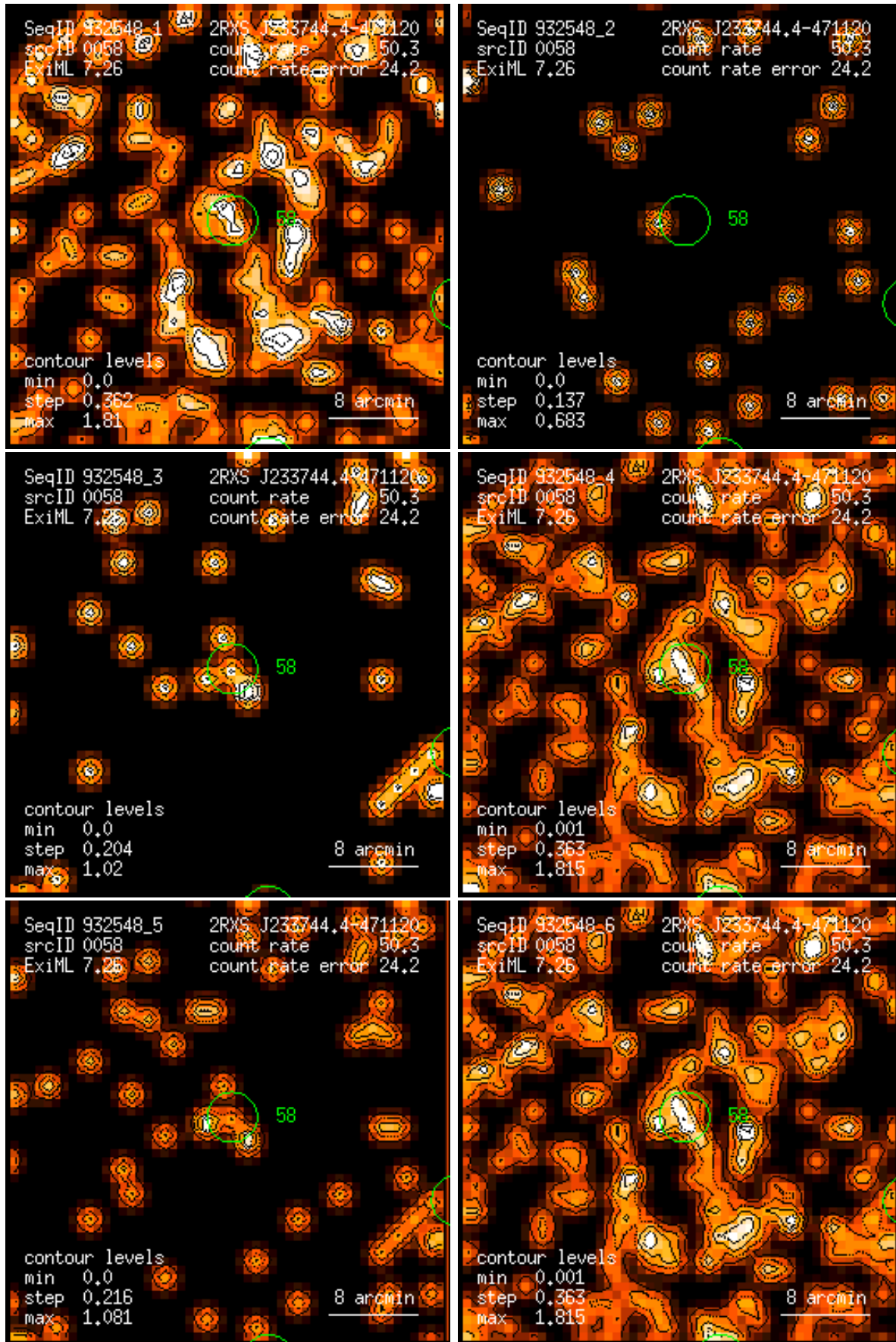
Figure 58: RASS 932548: detection 0058: band rate images, Gaussian filter: (1) PSPC channels 11 – 41, (2) 52 – 90, (3) 91 – 201, (4) 11 – 235, (5) 52 – 201, (6) 11 – 201. Broad band rates in counts/ks. Band rate contour levels in counts/ks/arcmin 2 .
