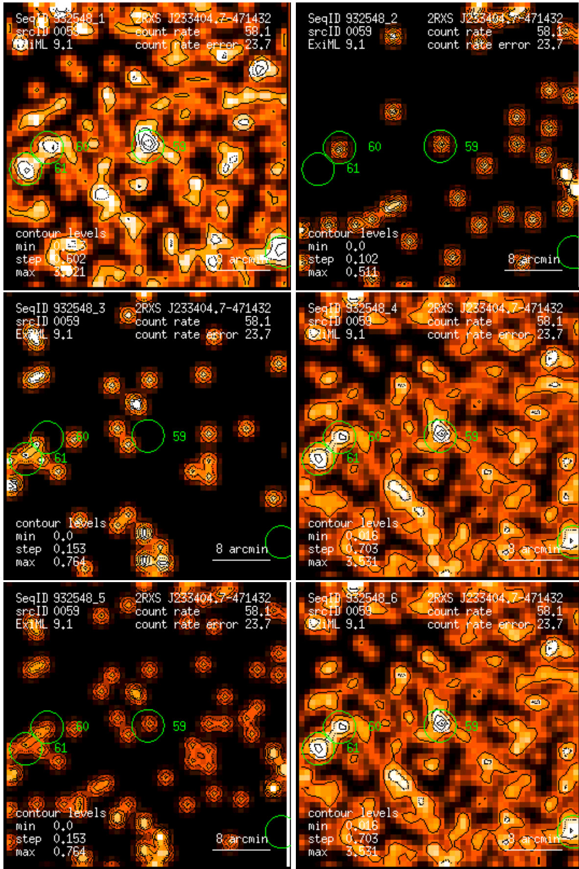
Figure 59: RASS 932548: detection 0059: band rate images, Gaussian filter: (1) PSPC channels 11 – 41, (2) 52 – 90, (3) 91 – 201, (4) 11 – 235, (5) 52 – 201, (6) 11 – 201. Broad band rates in counts/ks. Band rate contour levels in counts/ks/arcmin 2 .
