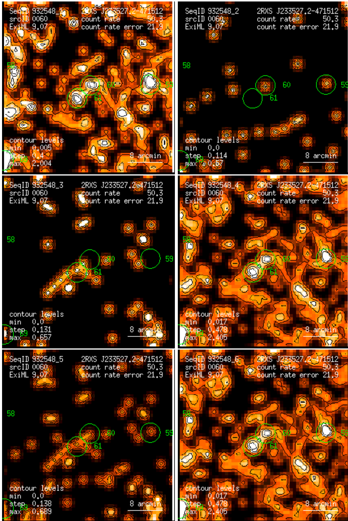
Figure 60: RASS 932548: detection 0060: band rate images, Gaussian filter: (1) PSPC channels 11 – 41, (2) 52 – 90, (3) 91 – 201, (4) 11 – 235, (5) 52 – 201, (6) 11 – 201. Broad band rates in counts/ks. Band rate contour levels in counts/ks/arcmin 2 .
