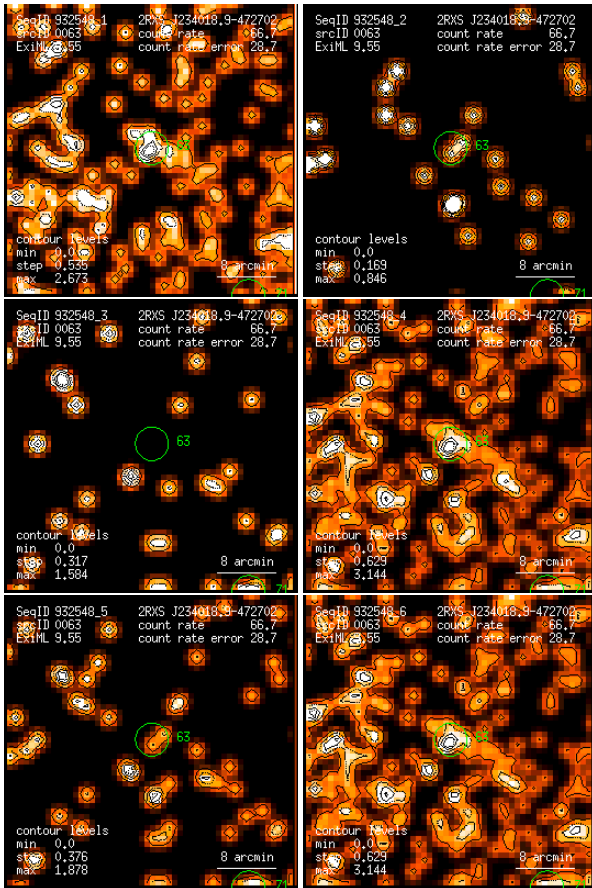
Figure 63: RASS 932548: detection 0063: band rate images, Gaussian filter: (1) PSPC channels 11 – 41, (2) 52 – 90, (3) 91 – 201, (4) 11 – 235, (5) 52 – 201, (6) 11 – 201. Broad band rates in counts/ks. Band rate contour levels in counts/ks/arcmin 2 .
