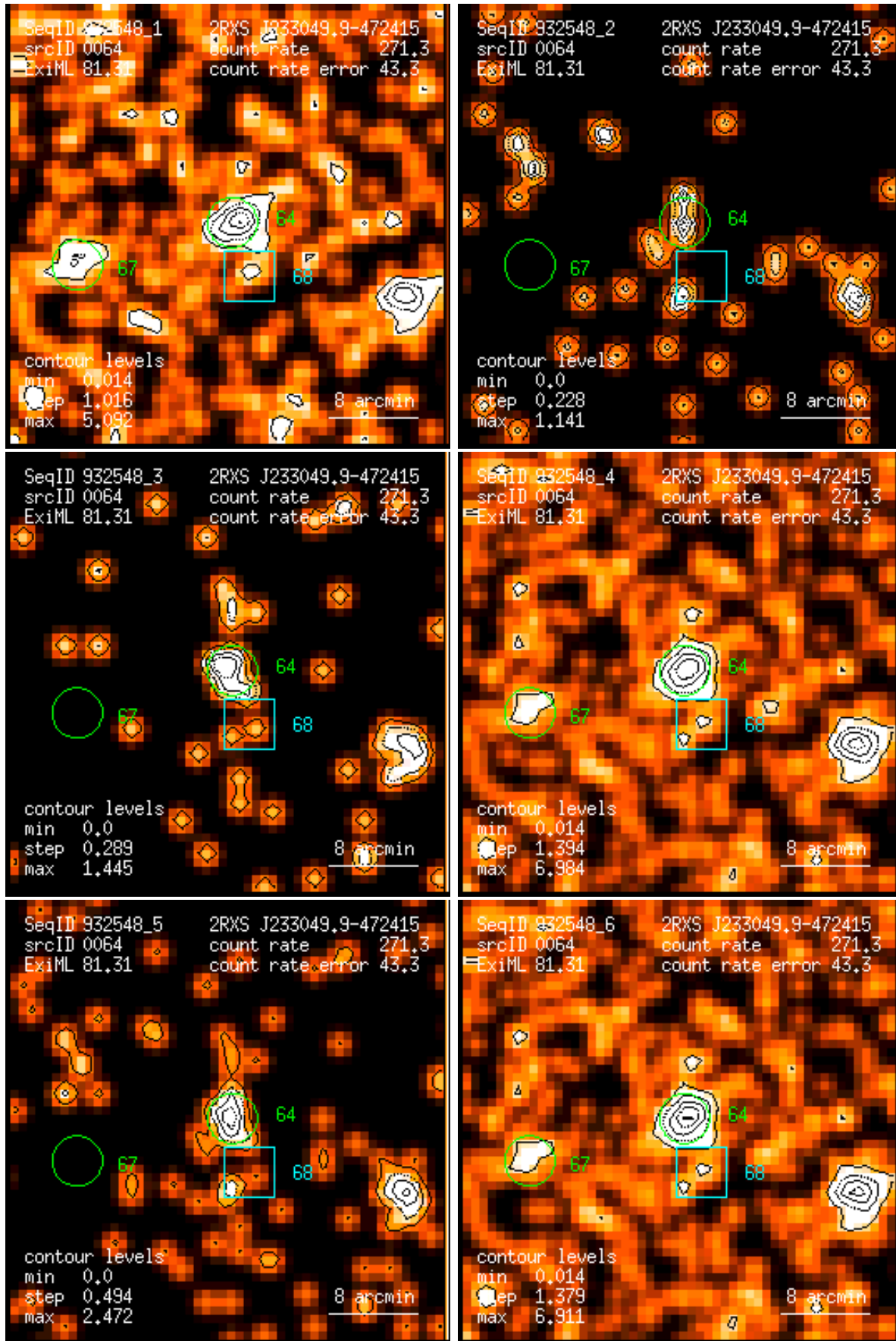
Figure 64: RASS 932548: detection 0064: band rate images, Gaussian filter: (1) PSPC channels 11 – 41, (2) 52 – 90, (3) 91 – 201, (4) 11 – 235, (5) 52 – 201, (6) 11 – 201. Broad band rates in counts/ks. Band rate contour levels in counts/ks/arcmin 2 .
