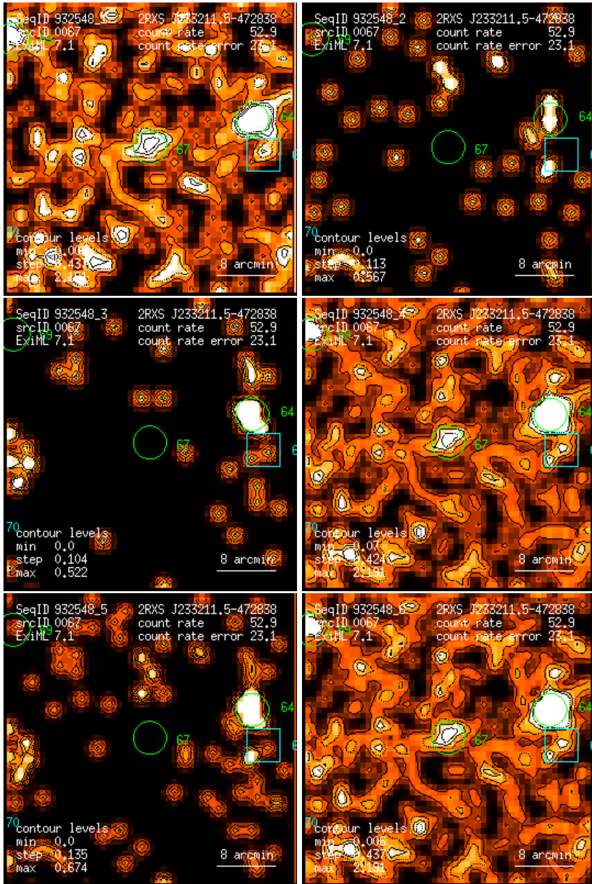
Figure 67: RASS 932548: detection 0067: band rate images, Gaussian filter: (1) PSPC channels 11 – 41, (2) 52 – 90, (3) 91 – 201, (4) 11 – 235, (5) 52 – 201, (6) 11 – 201. Broad band rates in counts/ks. Band rate contour levels in counts/ks/arcmin 2 .
