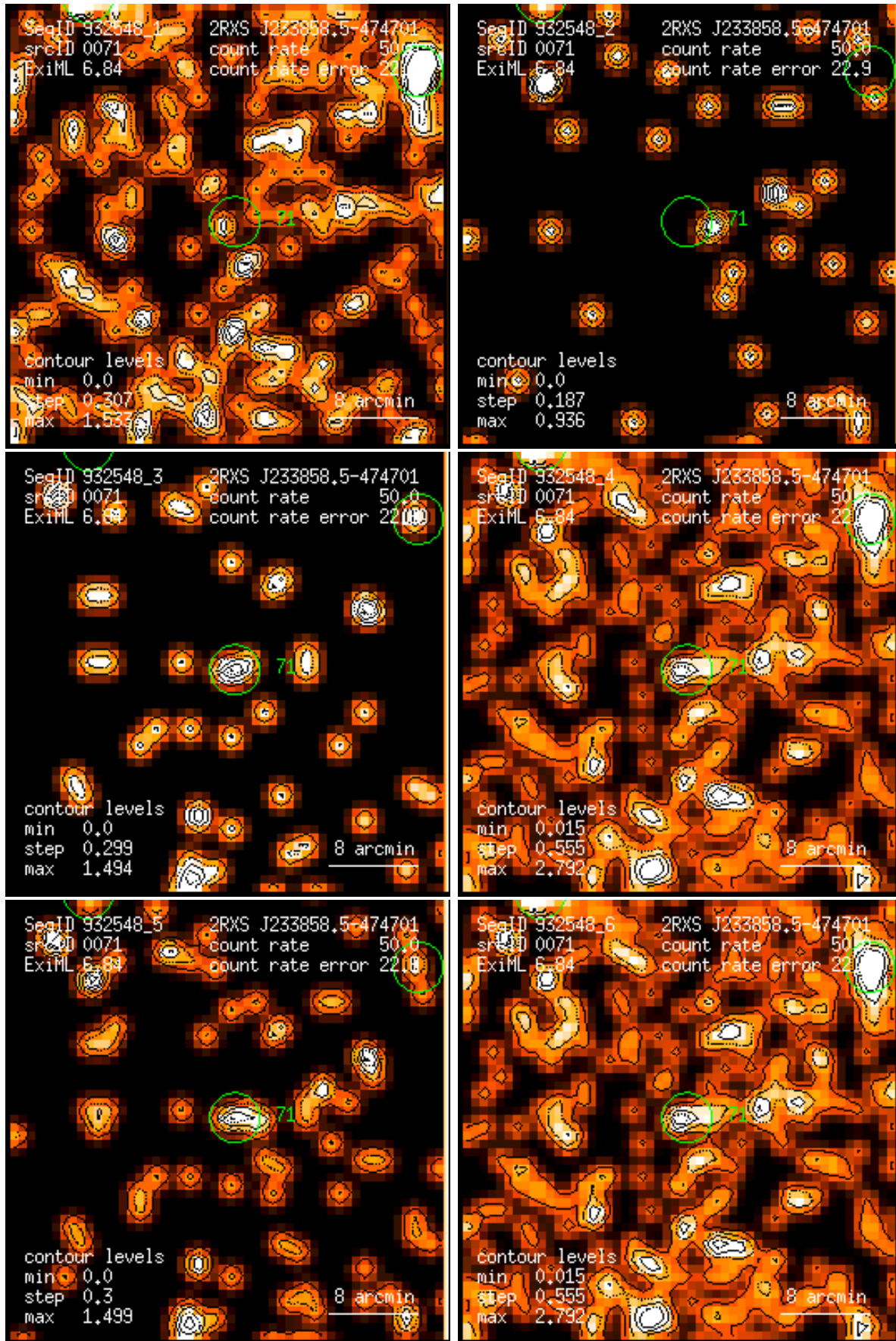
Figure 71: RASS 932548: detection 0071: band rate images, Gaussian filter: (1) PSPC channels 11 – 41, (2) 52 – 90, (3) 91 – 201, (4) 11 – 235, (5) 52 – 201, (6) 11 – 201. Broad band rates in counts/ks. Band rate contour levels in counts/ks/arcmin 2 .
