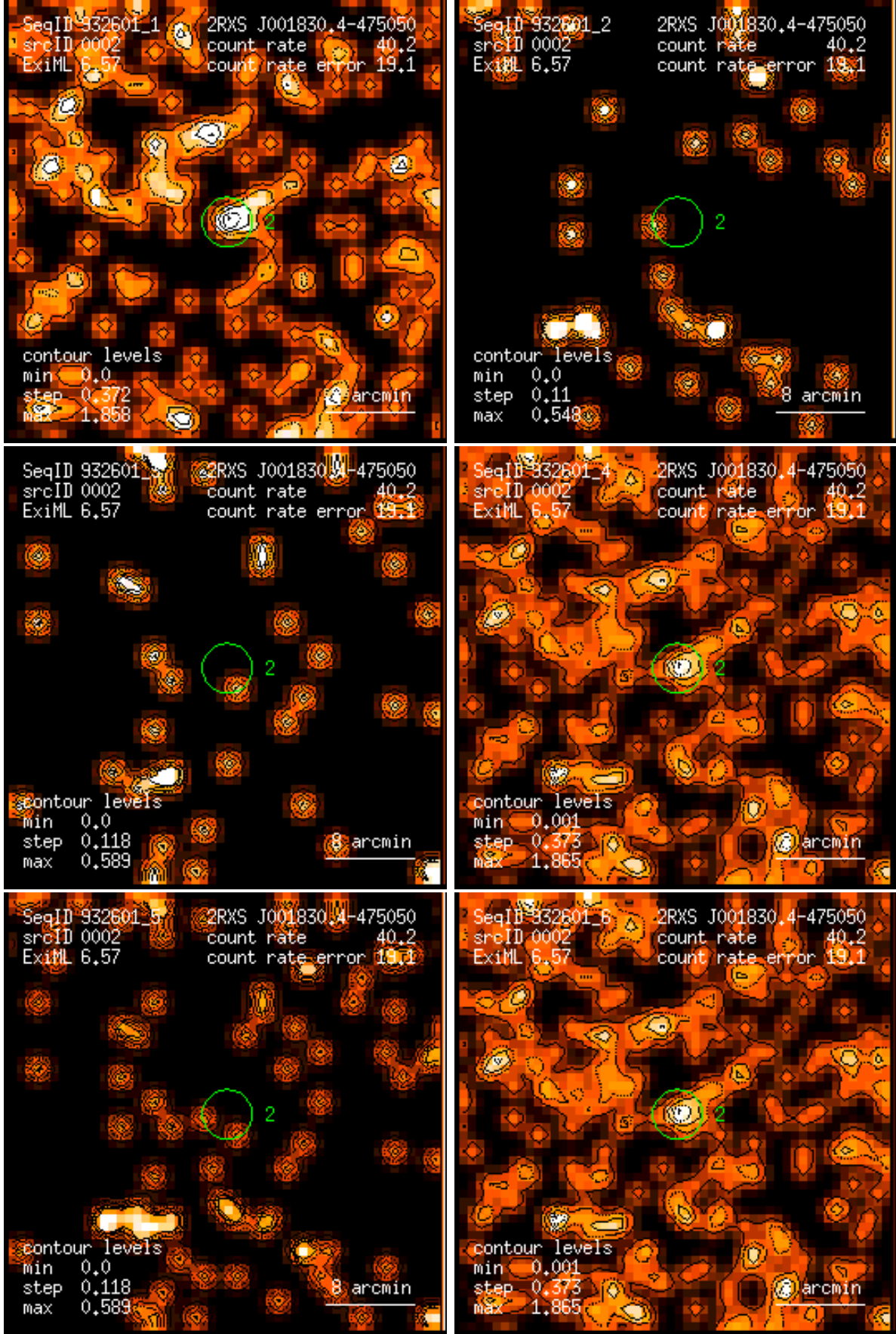
Figure 2: RASS 932601: detection 0002: band rate images, Gaussian filter: (1) PSPC channels 11 – 41, (2) 52 – 90, (3) 91 – 201, (4) 11 – 235, (5) 52 – 201, (6) 11 – 201. Broad band rates in counts/ks. Band rate contour levels in counts/ks/arcmin 2 .
