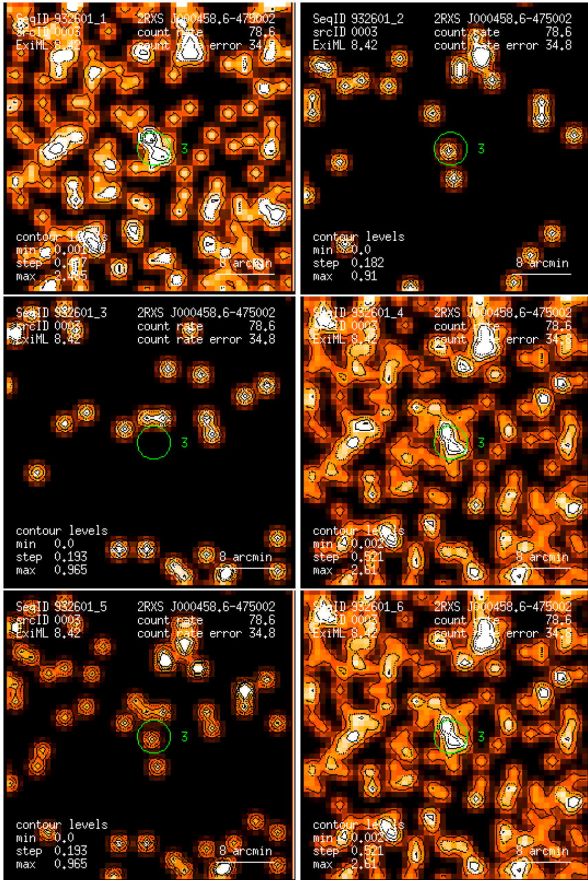
Figure 3: RASS 932601: detection 0003: band rate images, Gaussian filter: (1) PSPC channels 11 – 41, (2) 52 – 90, (3) 91 – 201, (4) 11 – 235, (5) 52 – 201, (6) 11 – 201. Broad band rates in counts/ks. Band rate contour levels in counts/ks/arcmin 2 .
