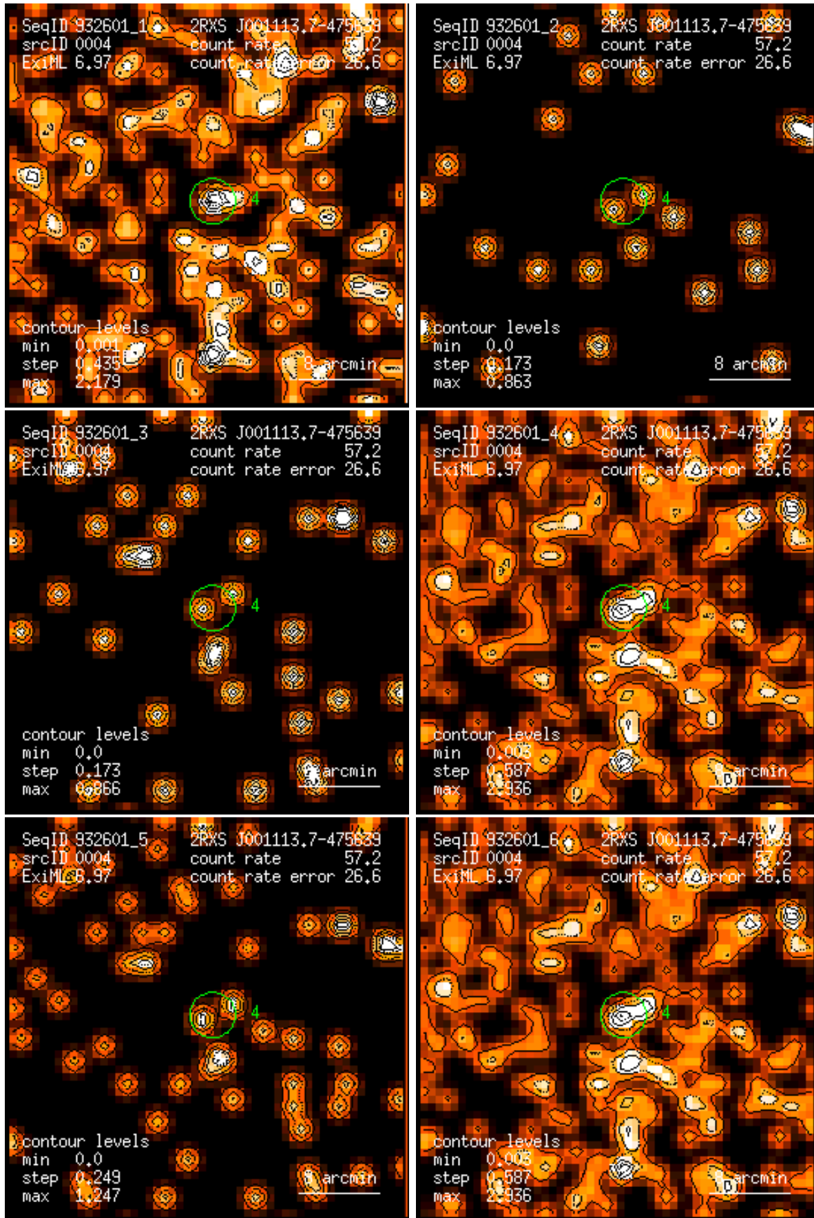
Figure 4: RASS 932601: detection 0004: band rate images, Gaussian filter: (1) PSPC channels 11 – 41, (2) 52 – 90, (3) 91 – 201, (4) 11 – 235, (5) 52 – 201, (6) 11 – 201. Broad band rates in counts/ks. Band rate contour levels in counts/ks/arcmin 2 .
