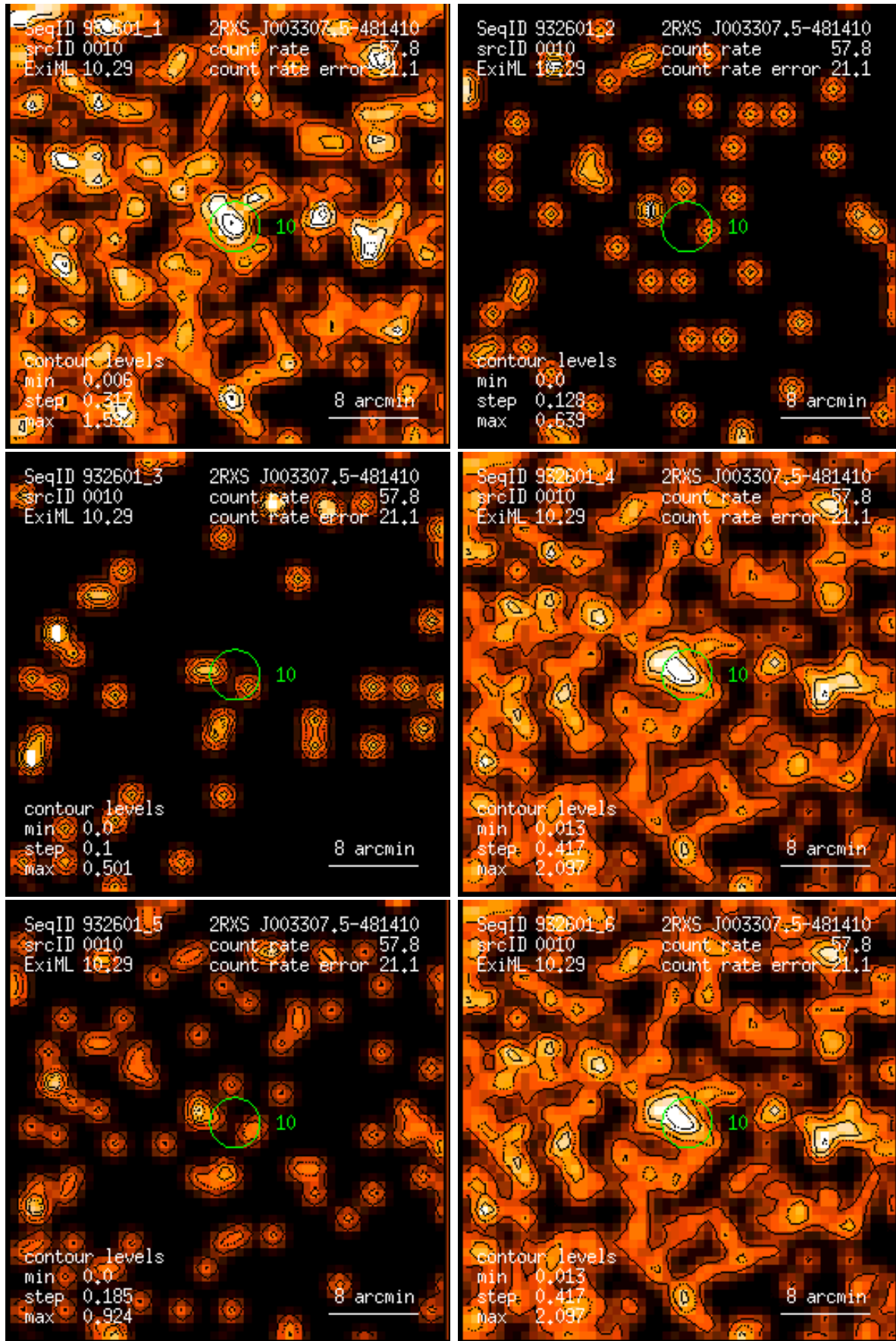
Figure 10: RASS 932601: detection 0010: band rate images, Gaussian filter: (1) PSPC channels 11 – 41, (2) 52 – 90, (3) 91 – 201, (4) 11 – 235, (5) 52 – 201, (6) 11 – 201. Broad band rates in counts/ks. Band rate contour levels in counts/ks/arcmin 2 .
