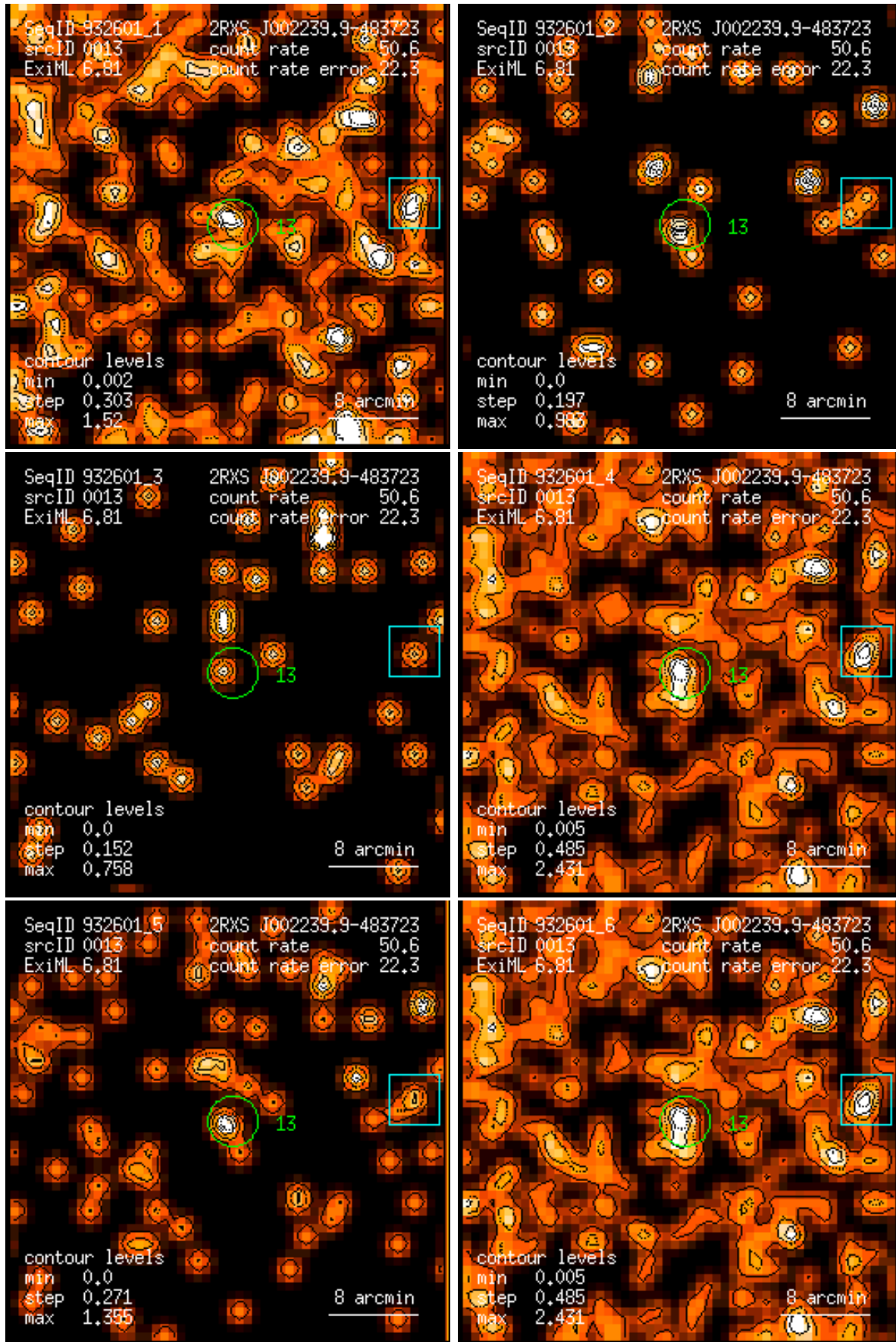
Figure 13: RASS 932601: detection 0013: band rate images, Gaussian filter: (1) PSPC channels 11 – 41, (2) 52 – 90, (3) 91 – 201, (4) 11 – 235, (5) 52 – 201, (6) 11 – 201. Broad band rates in counts/ks. Band rate contour levels in counts/ks/arcmin 2 .
