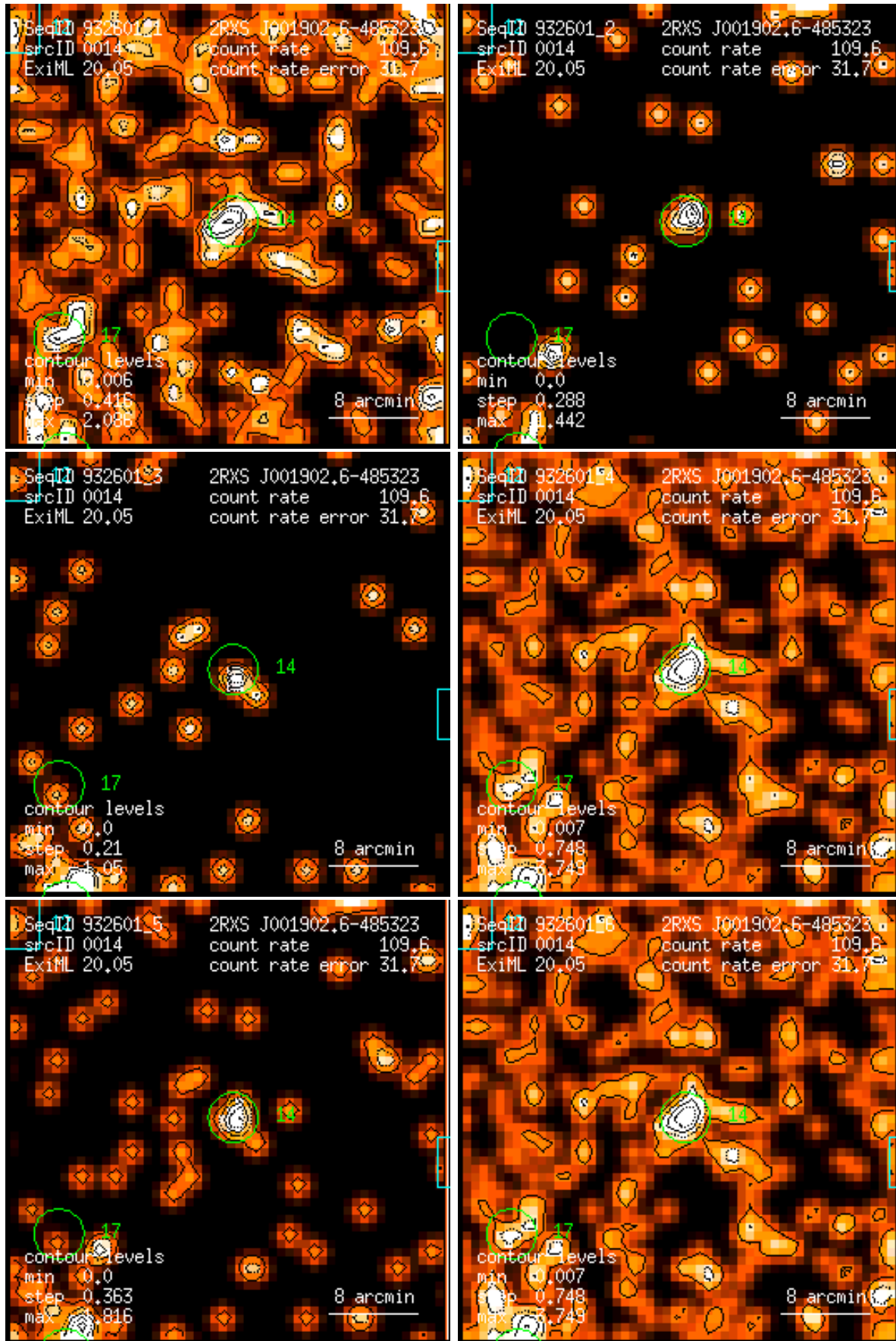
Figure 14: RASS 932601: detection 0014: band rate images, Gaussian filter: (1) PSPC channels 11 – 41, (2) 52 – 90, (3) 91 – 201, (4) 11 – 235, (5) 52 – 201, (6) 11 – 201. Broad band rates in counts/ks. Band rate contour levels in counts/ks/arcmin 2 .
