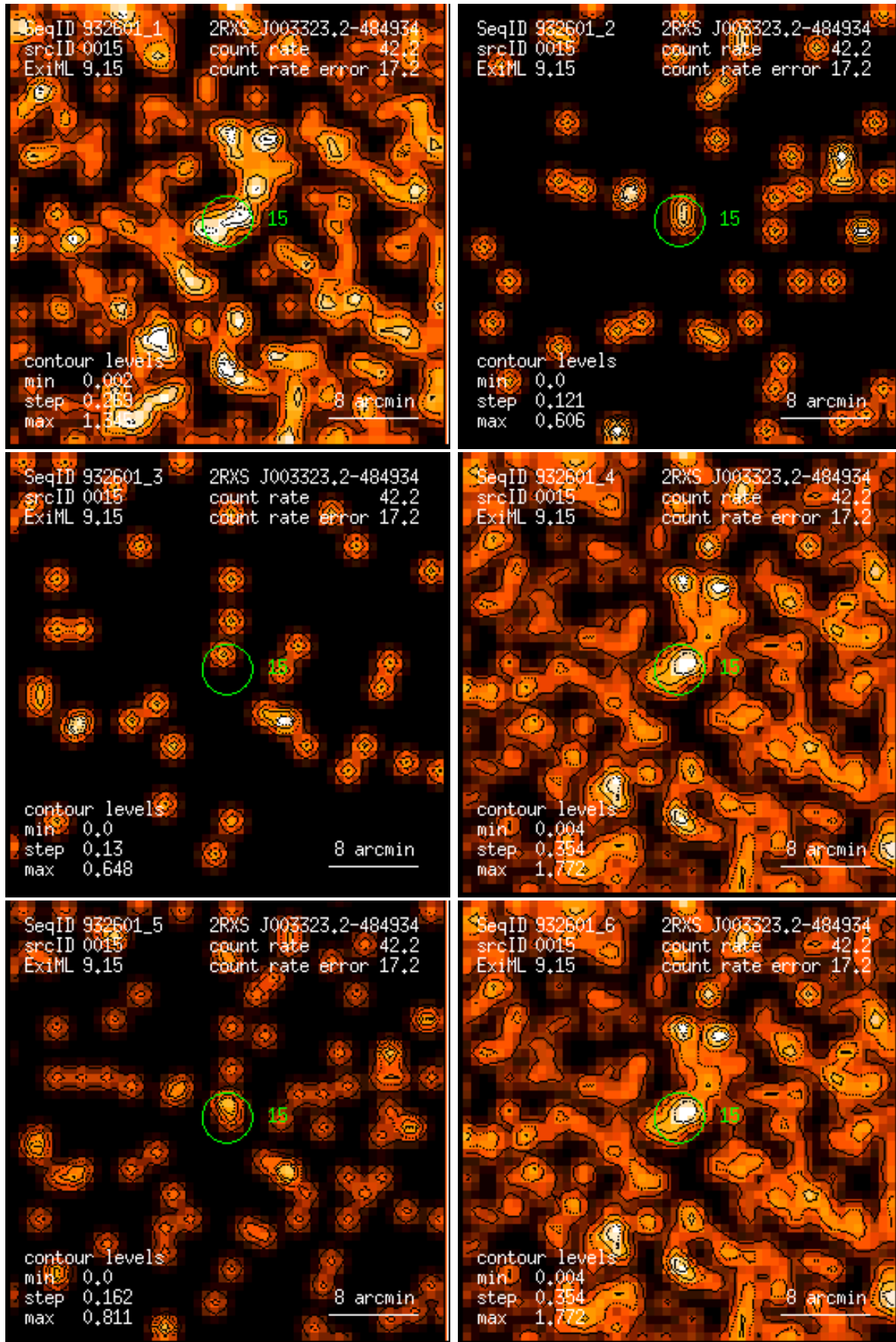
Figure 15: RASS 932601: detection 0015: band rate images, Gaussian filter: (1) PSPC channels 11 – 41, (2) 52 – 90, (3) 91 – 201, (4) 11 – 235, (5) 52 – 201, (6) 11 – 201. Broad band rates in counts/ks. Band rate contour levels in counts/ks/arcmin 2 .
