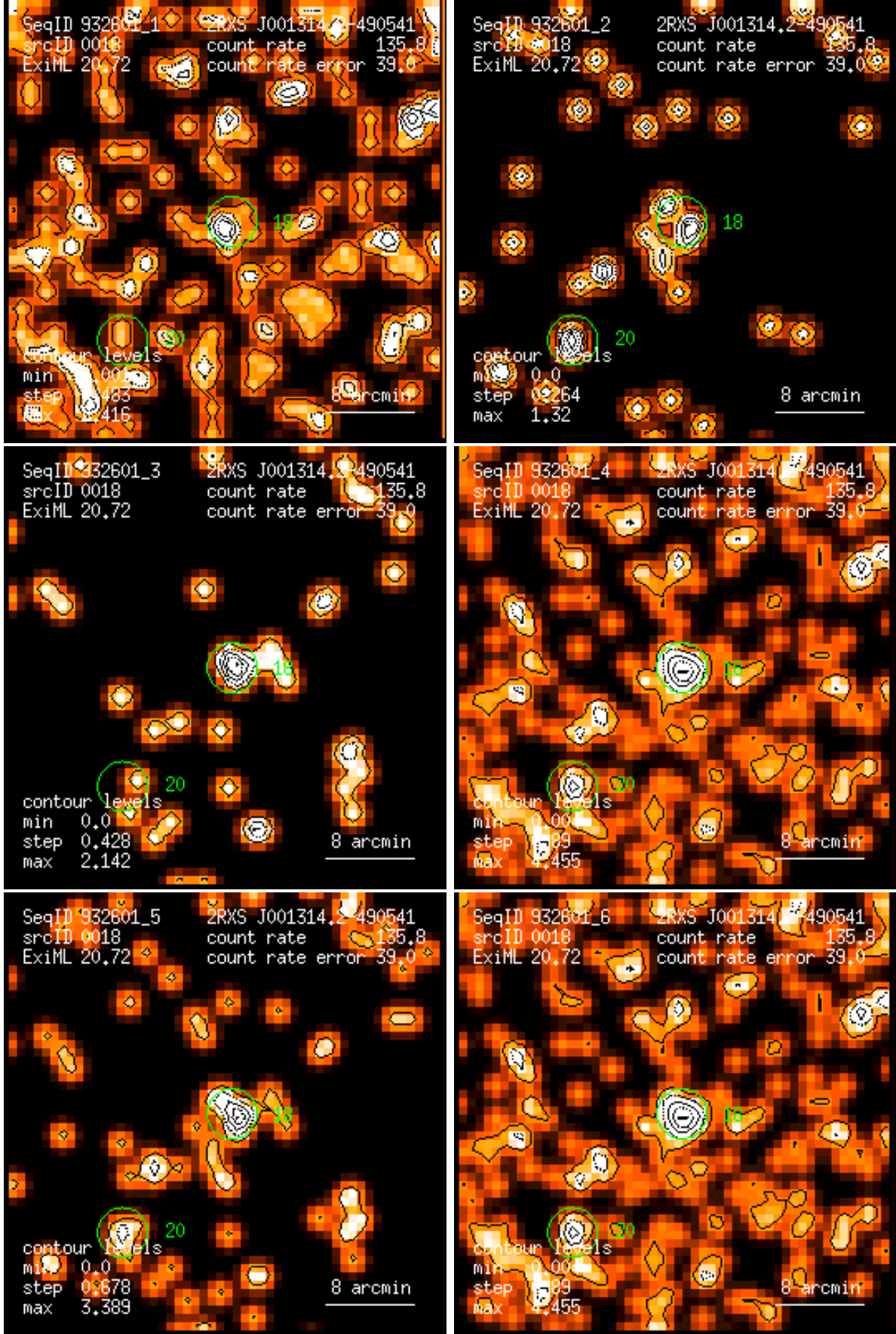
Figure 18: RASS 932601: detection 0018: band rate images, Gaussian filter: (1) PSPC channels 11 – 41, (2) 52 – 90, (3) 91 – 201, (4) 11 – 235, (5) 52 – 201, (6) 11 – 201. Broad band rates in counts/ks. Band rate contour levels in counts/ks/arcmin 2 .
