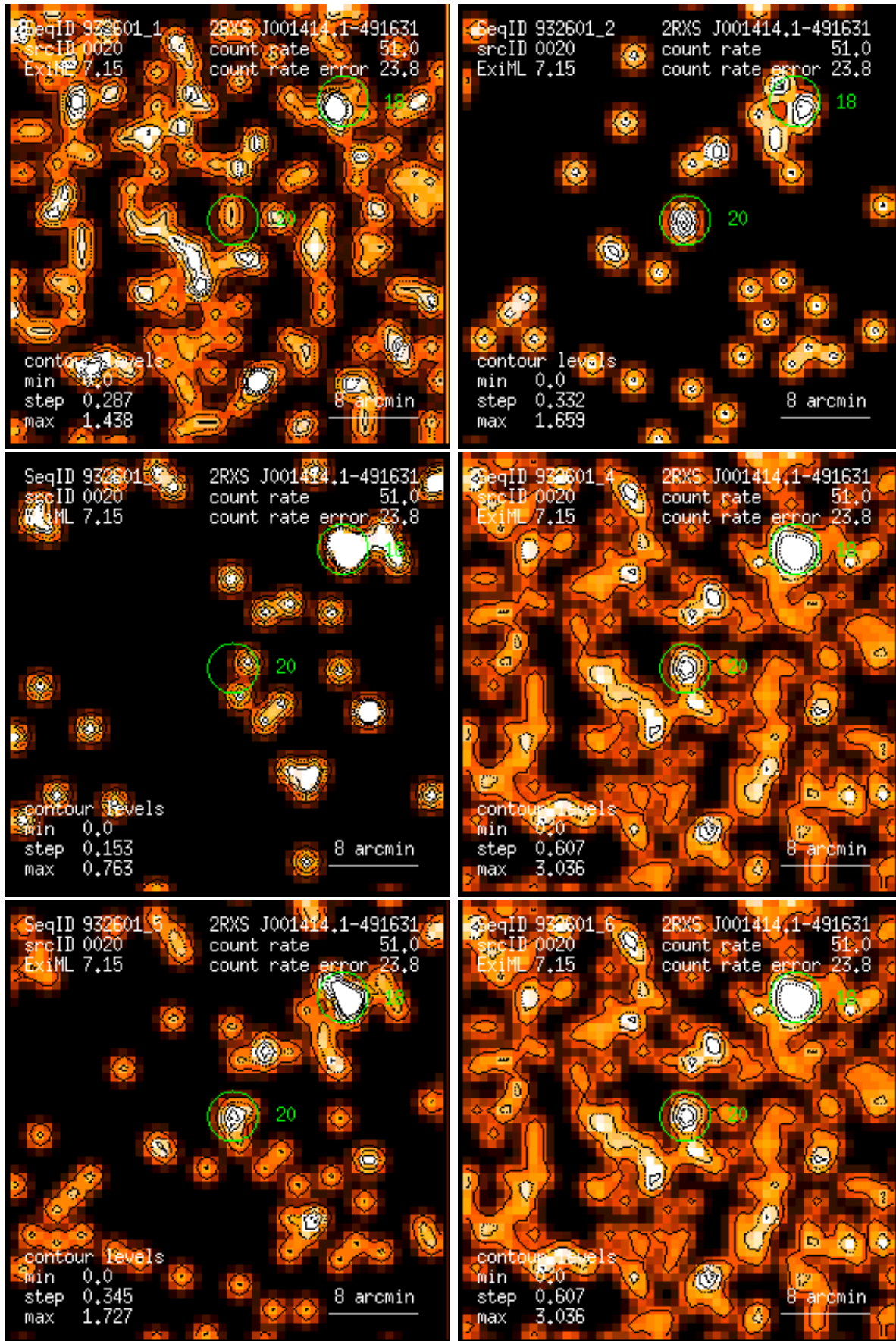
Figure 20: RASS 932601: detection 0020: band rate images, Gaussian filter: (1) PSPC channels 11 – 41, (2) 52 – 90, (3) 91 – 201, (4) 11 – 235, (5) 52 – 201, (6) 11 – 201. Broad band rates in counts/ks. Band rate contour levels in counts/ks/arcmin 2 .
