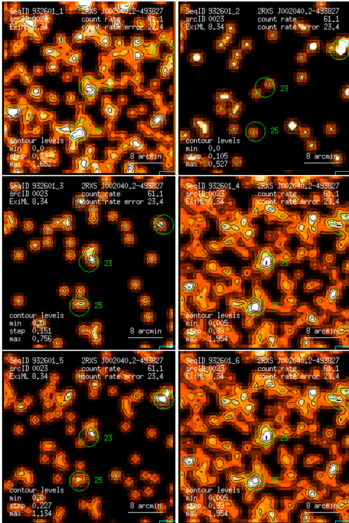
Figure 23: RASS 932601: detection 0023: band rate images, Gaussian filter: (1) PSPC channels 11 – 41, (2) 52 – 90, (3) 91 – 201, (4) 11 – 235, (5) 52 – 201, (6) 11 – 201. Broad band rates in counts/ks. Band rate contour levels in counts/ks/arcmin 2 .
