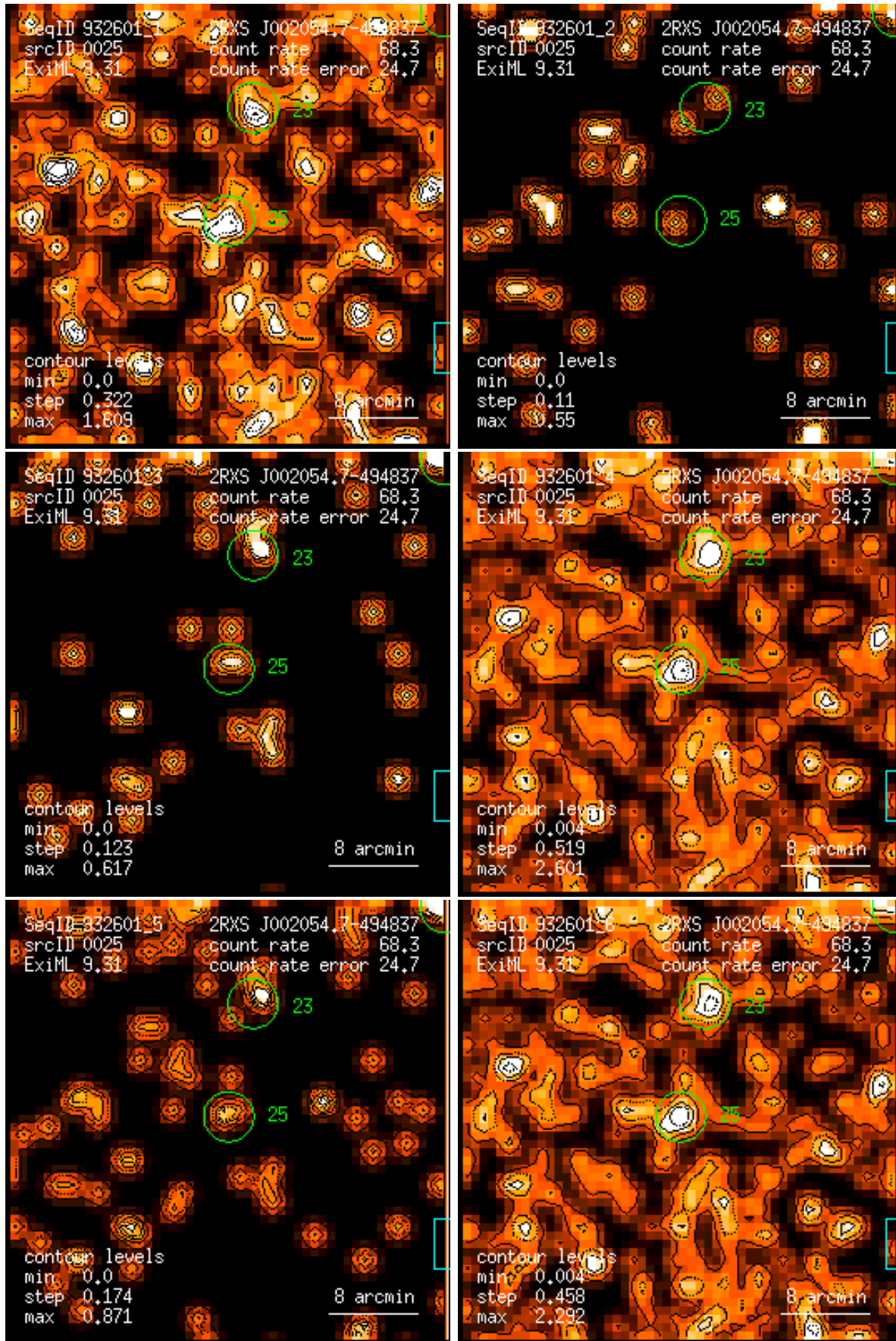
Figure 25: RASS 932601: detection 0025: band rate images, Gaussian filter: (1) PSPC channels 11 – 41, (2) 52 – 90, (3) 91 – 201, (4) 11 – 235, (5) 52 – 201, (6) 11 – 201. Broad band rates in counts/ks. Band rate contour levels in counts/ks/arcmin 2 .
