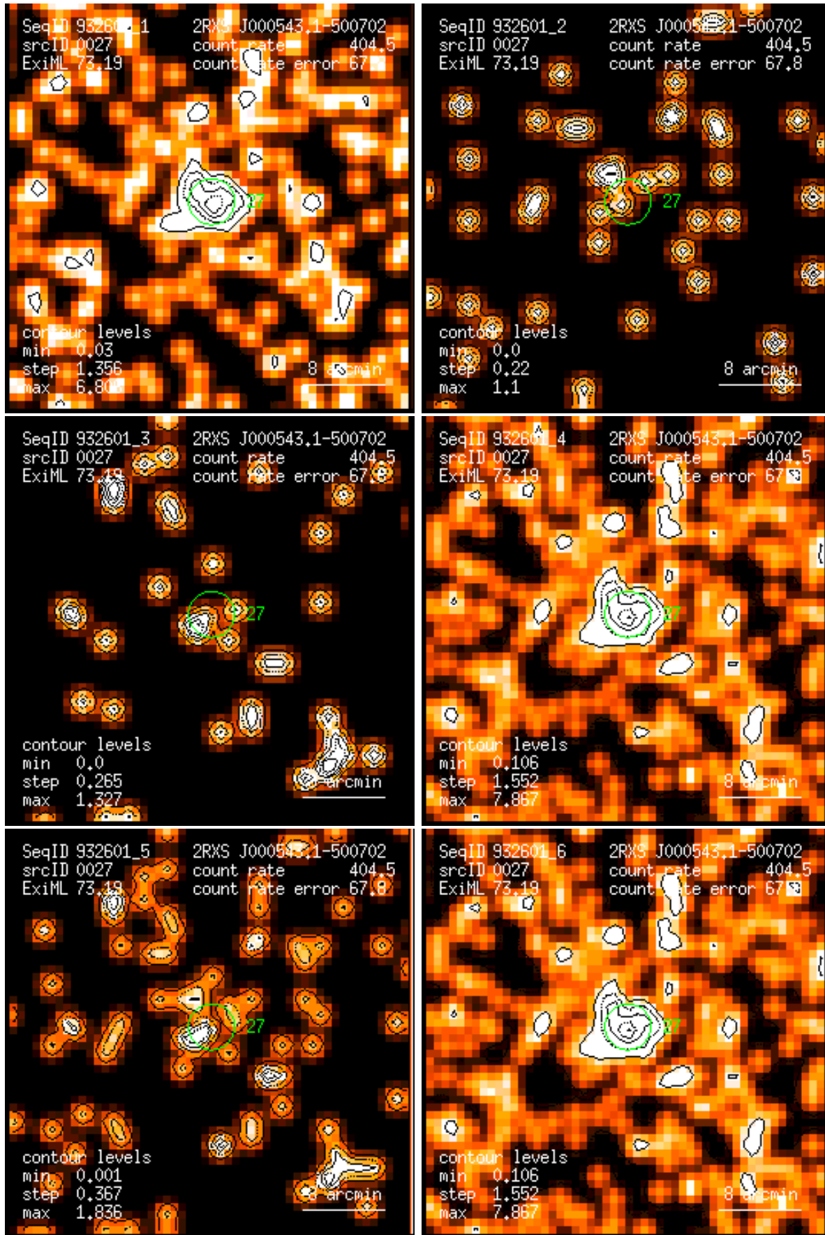
Figure 27: RASS 932601: detection 0027: band rate images, Gaussian filter: (1) PSPC channels 11 – 41, (2) 52 – 90, (3) 91 – 201, (4) 11 – 235, (5) 52 – 201, (6) 11 – 201. Broad band rates in counts/ks. Band rate contour levels in counts/ks/arcmin 2 .
