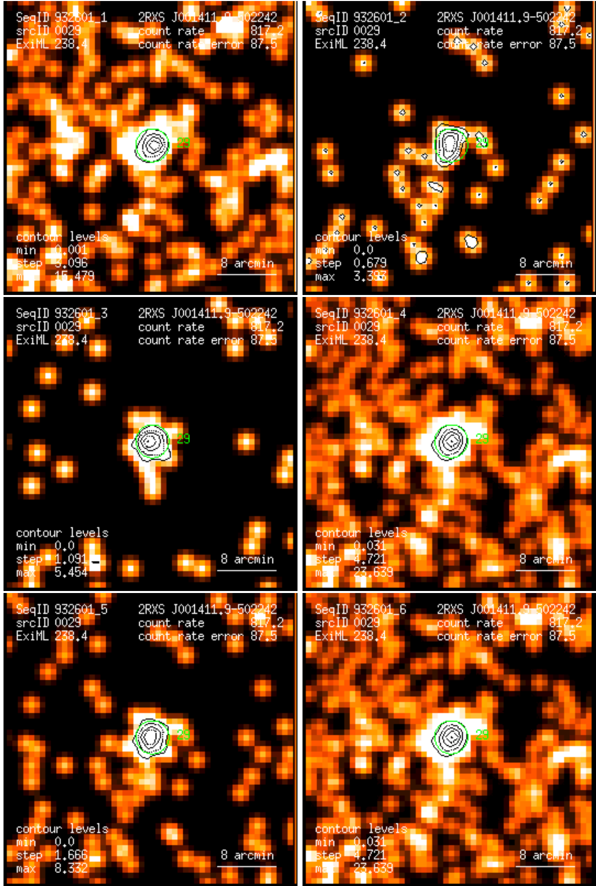
Figure 29: RASS 932601: detection 0029: band rate images, Gaussian filter: (1) PSPC channels 11 – 41, (2) 52 – 90, (3) 91 – 201, (4) 11 – 235, (5) 52 – 201, (6) 11 – 201. Broad band rates in counts/ks. Band rate contour levels in counts/ks/arcmin 2 .
