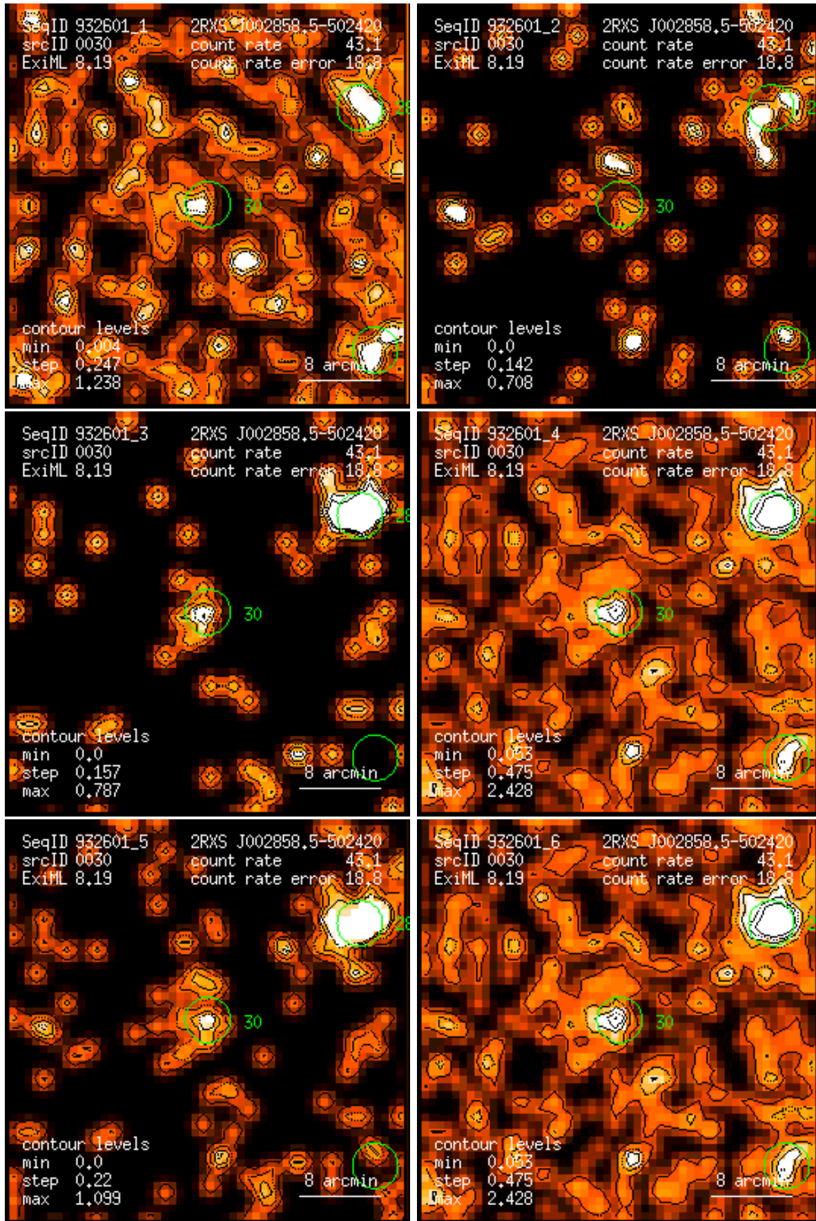
Figure 30: RASS 932601: detection 0030: band rate images, Gaussian filter: (1) PSPC channels 11 – 41, (2) 52 – 90, (3) 91 – 201, (4) 11 – 235, (5) 52 – 201, (6) 11 – 201. Broad band rates in counts/ks. Band rate contour levels in counts/ks/arcmin 2 .
