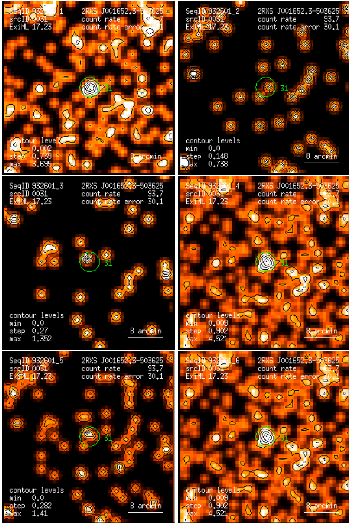
Figure 31: RASS 932601: detection 0031: band rate images, Gaussian filter: (1) PSPC channels 11 – 41, (2) 52 – 90, (3) 91 – 201, (4) 11 – 235, (5) 52 – 201, (6) 11 – 201. Broad band rates in counts/ks. Band rate contour levels in counts/ks/arcmin 2 .
