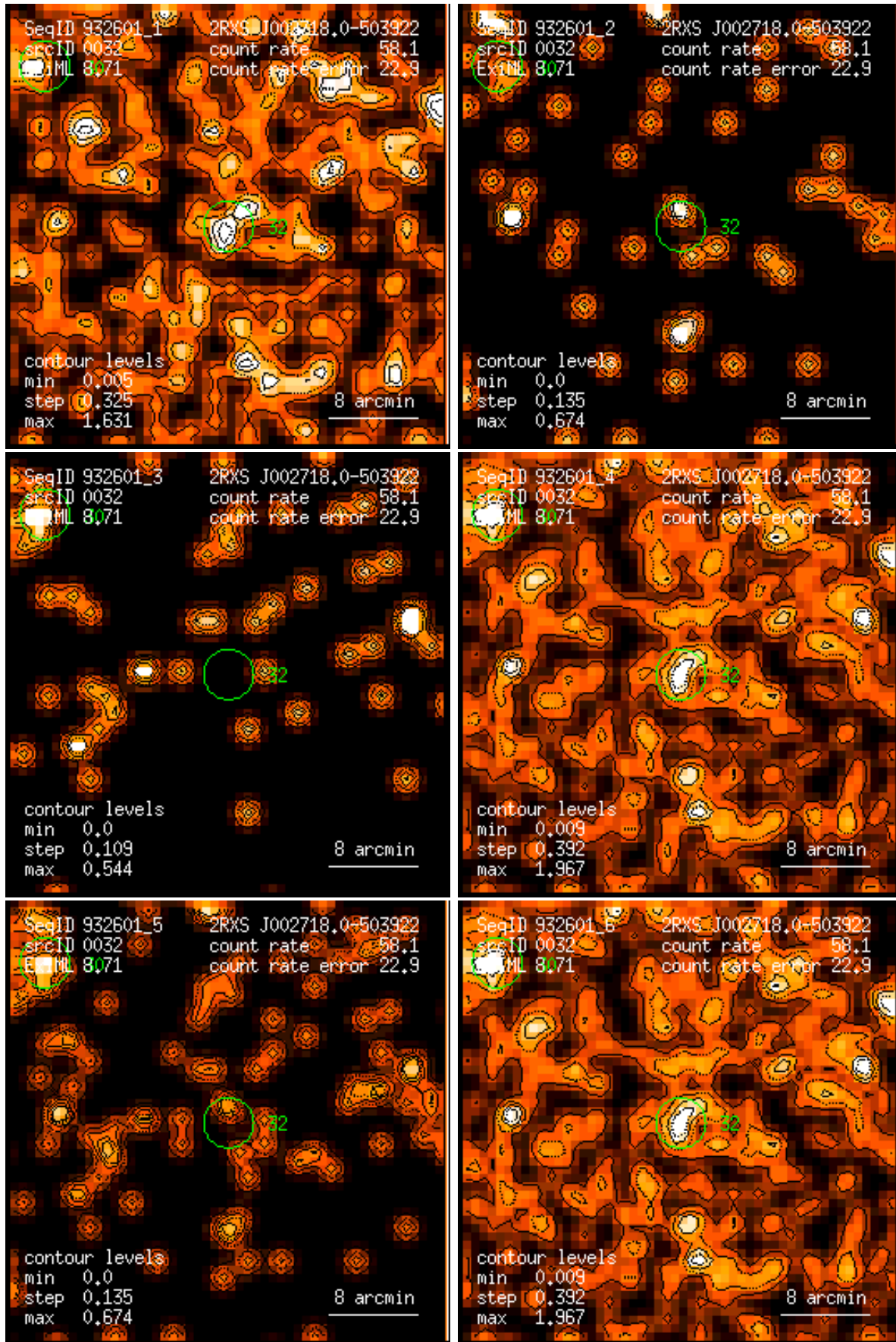
Figure 32: RASS 932601: detection 0032: band rate images, Gaussian filter: (1) PSPC channels 11 – 41, (2) 52 – 90, (3) 91 – 201, (4) 11 – 235, (5) 52 – 201, (6) 11 – 201. Broad band rates in counts/ks. Band rate contour levels in counts/ks/arcmin 2 .
