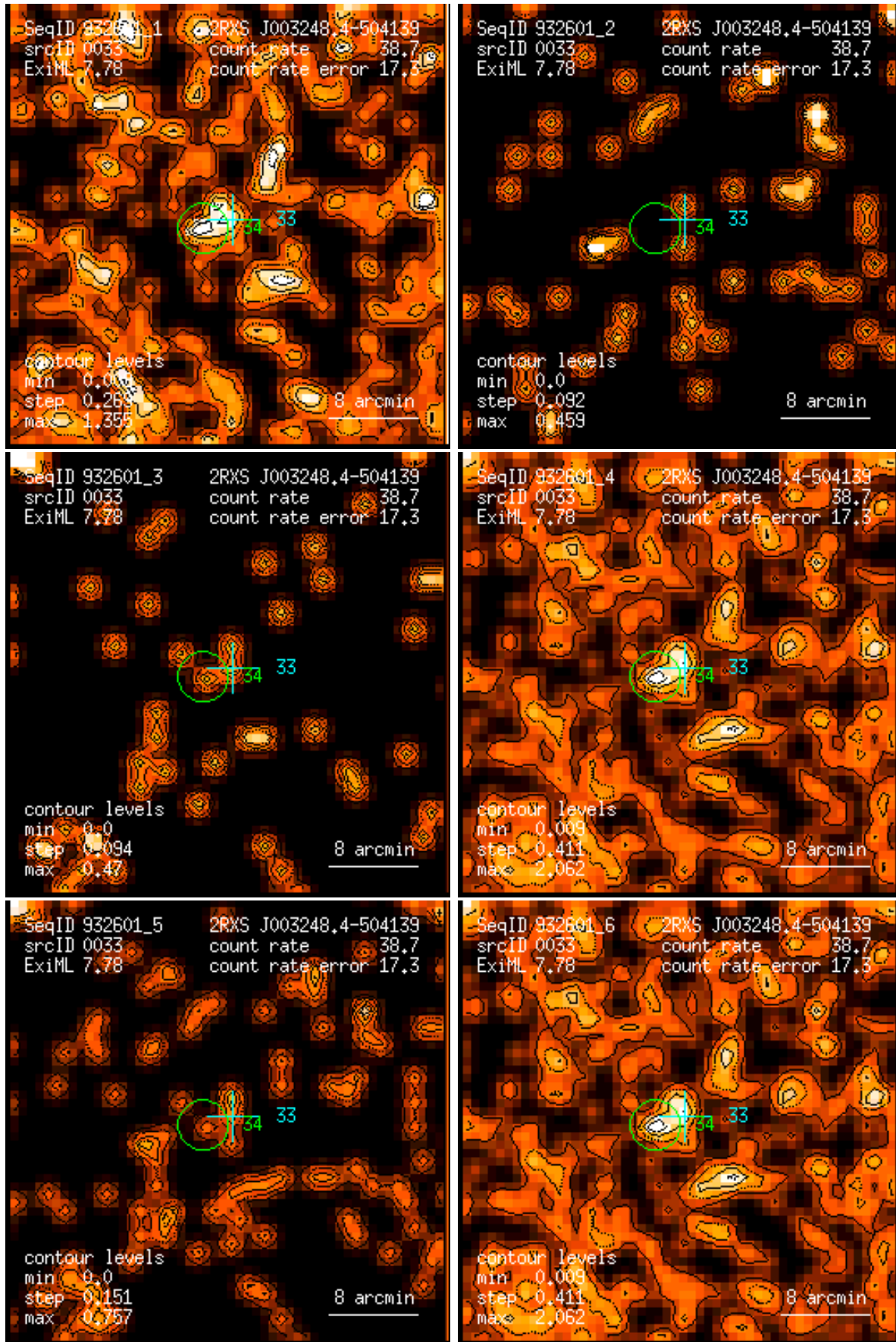
Figure 33: RASS 932601: detection 0033: band rate images, Gaussian filter: (1) PSPC channels 11 – 41, (2) 52 – 90, (3) 91 – 201, (4) 11 – 235, (5) 52 – 201, (6) 11 – 201. Broad band rates in counts/ks. Band rate contour levels in counts/ks/arcmin 2 .
