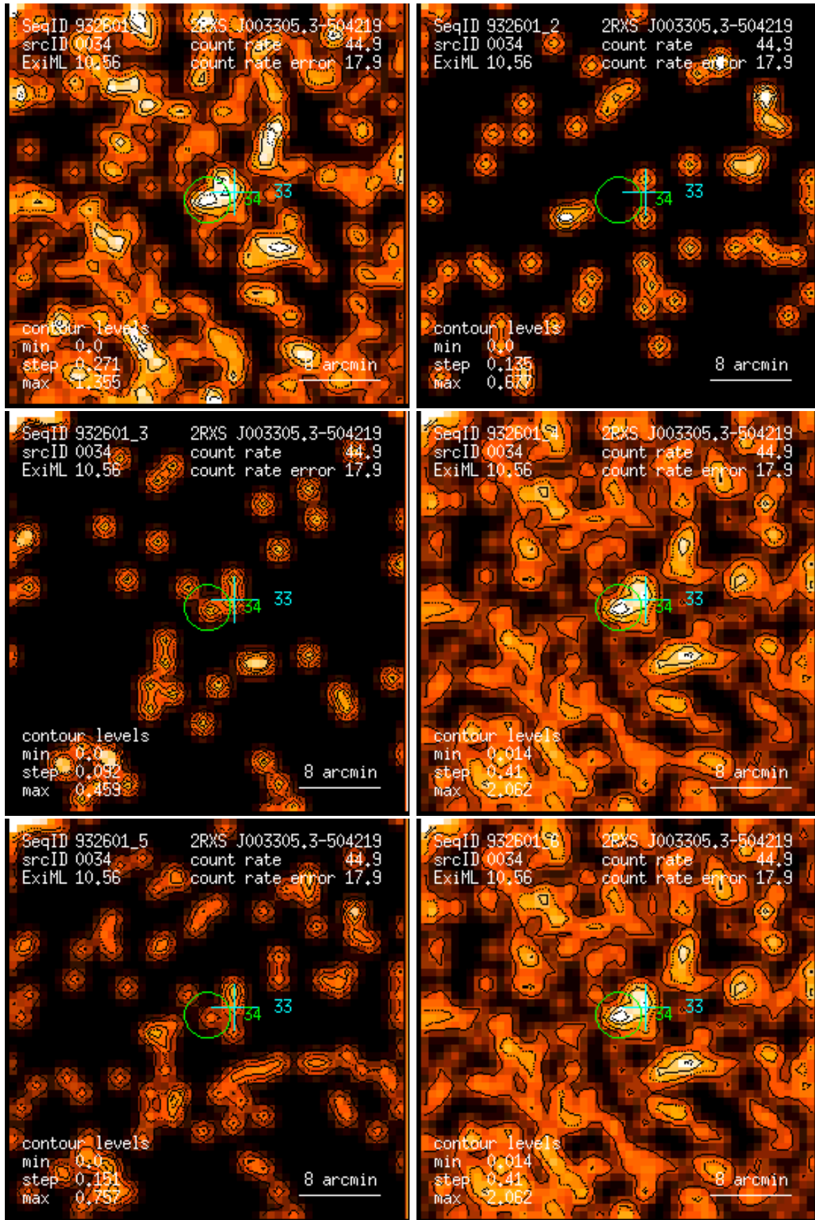
Figure 34: RASS 932601: detection 0034: band rate images, Gaussian filter: (1) PSPC channels 11 – 41, (2) 52 – 90, (3) 91 – 201, (4) 11 – 235, (5) 52 – 201, (6) 11 – 201. Broad band rates in counts/ks. Band rate contour levels in counts/ks/arcmin 2 .
