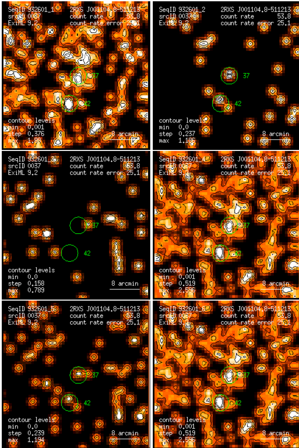
Figure 37: RASS 932601: detection 0037: band rate images, Gaussian filter: (1) PSPC channels 11 – 41, (2) 52 – 90, (3) 91 – 201, (4) 11 – 235, (5) 52 – 201, (6) 11 – 201. Broad band rates in counts/ks. Band rate contour levels in counts/ks/arcmin 2 .
