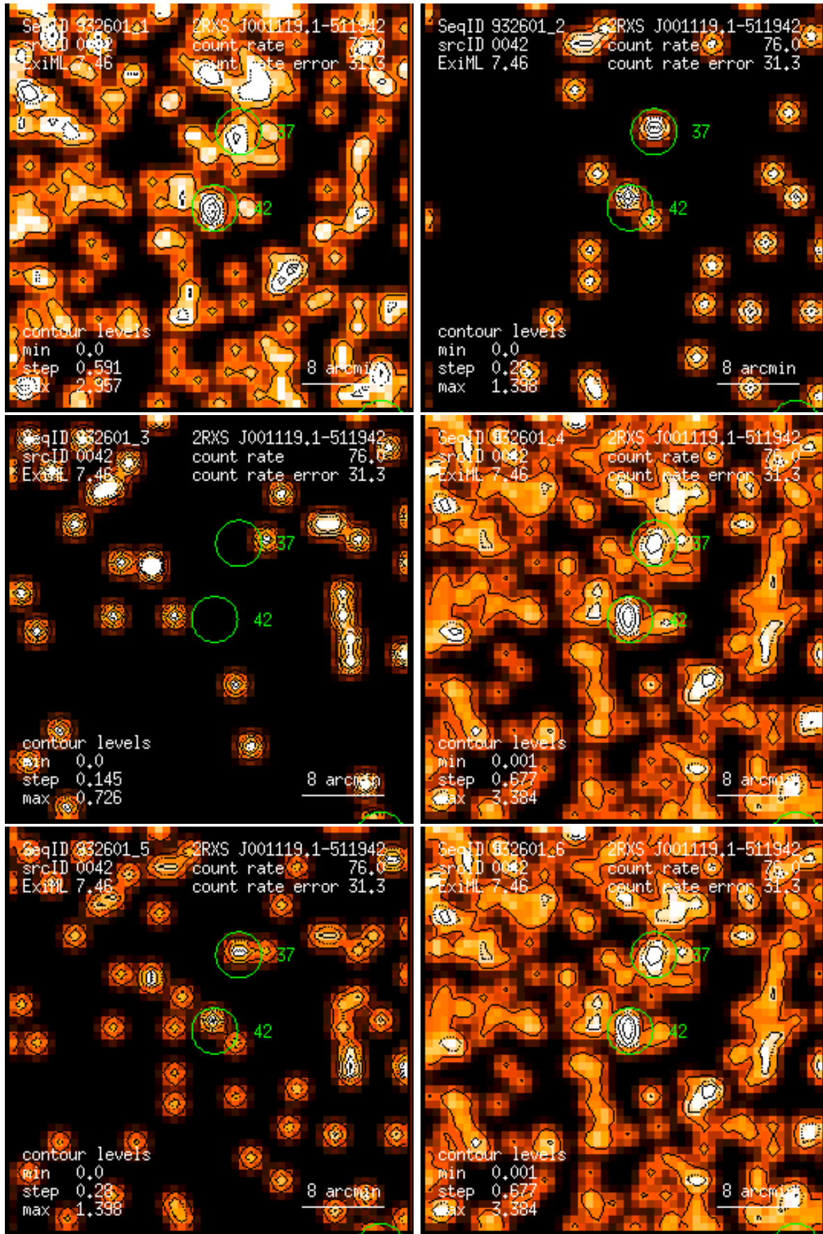
Figure 42: RASS 932601: detection 0042: band rate images, Gaussian filter: (1) PSPC channels 11 – 41, (2) 52 – 90, (3) 91 – 201, (4) 11 – 235, (5) 52 – 201, (6) 11 – 201. Broad band rates in counts/ks. Band rate contour levels in counts/ks/arcmin 2 .
