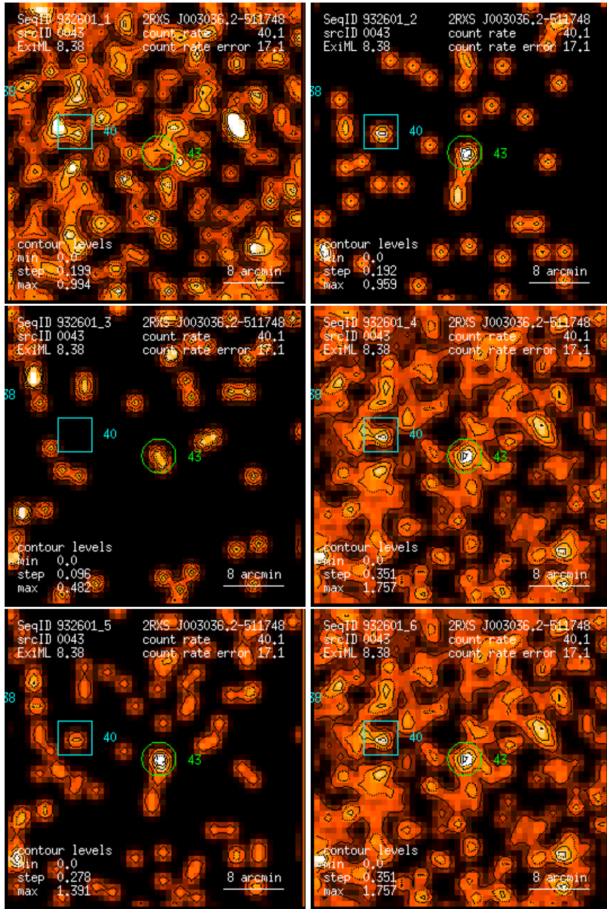
Figure 43: RASS 932601: detection 0043: band rate images, Gaussian filter: (1) PSPC channels 11 – 41, (2) 52 – 90, (3) 91 – 201, (4) 11 – 235, (5) 52 – 201, (6) 11 – 201. Broad band rates in counts/ks. Band rate contour levels in counts/ks/arcmin 2 .
