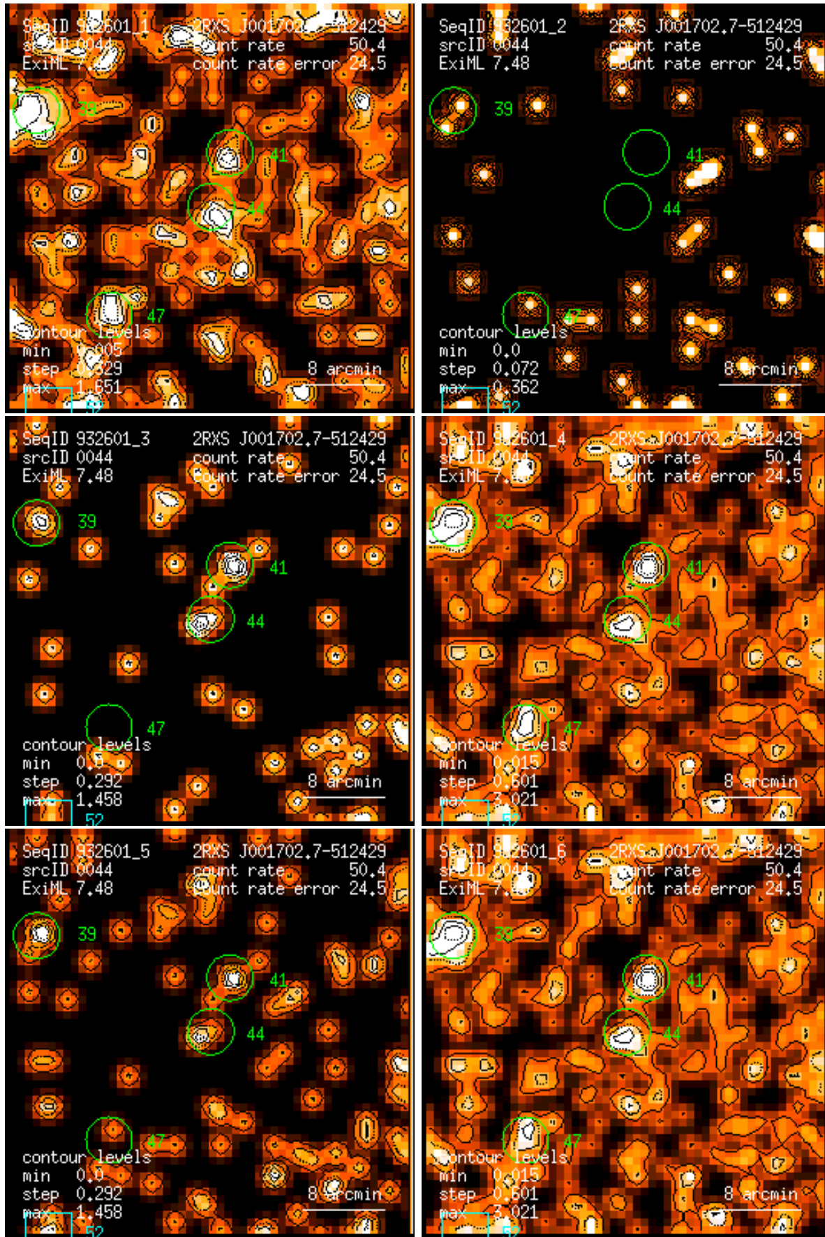
Figure 44: RASS 932601: detection 0044: band rate images, Gaussian filter: (1) PSPC channels 11 – 41, (2) 52 – 90, (3) 91 – 201, (4) 11 – 235, (5) 52 – 201, (6) 11 – 201. Broad band rates in counts/ks. Band rate contour levels in counts/ks/arcmin 2 .
