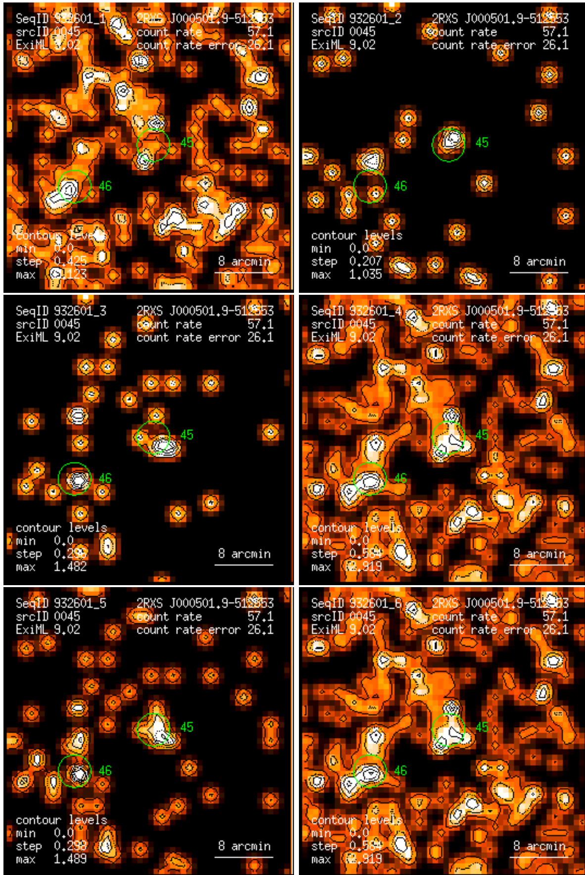
Figure 45: RASS 932601: detection 0045: band rate images, Gaussian filter: (1) PSPC channels 11 – 41, (2) 52 – 90, (3) 91 – 201, (4) 11 – 235, (5) 52 – 201, (6) 11 – 201. Broad band rates in counts/ks. Band rate contour levels in counts/ks/arcmin 2 .
