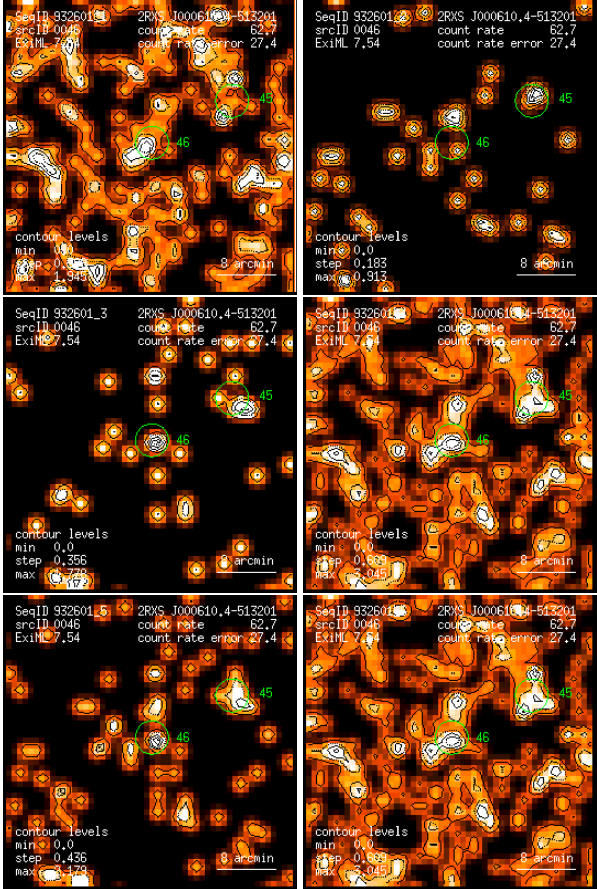
Figure 46: RASS 932601: detection 0046: band rate images, Gaussian filter: (1) PSPC channels 11 – 41, (2) 52 – 90, (3) 91 – 201, (4) 11 – 235, (5) 52 – 201, (6) 11 – 201. Broad band rates in counts/ks. Band rate contour levels in counts/ks/arcmin 2 .
