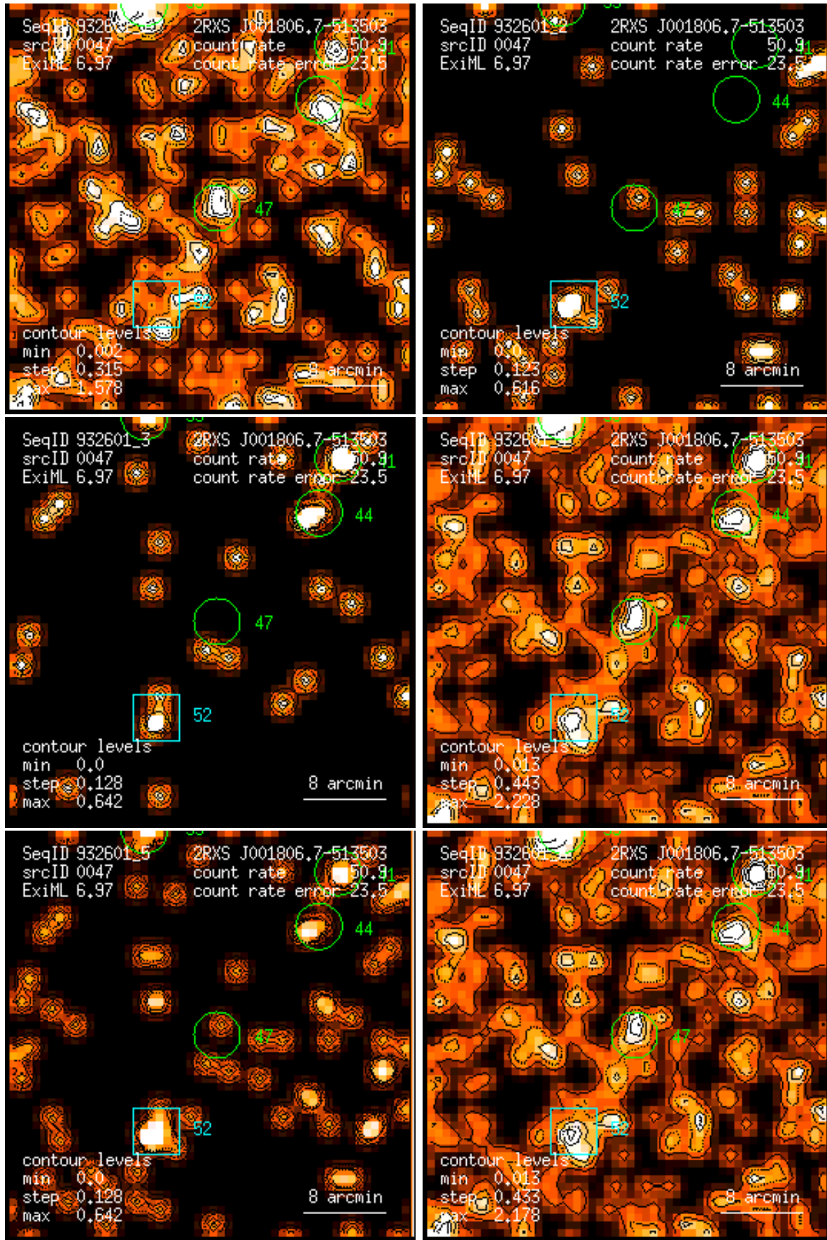
Figure 47: RASS 932601: detection 0047: band rate images, Gaussian filter: (1) PSPC channels 11 – 41, (2) 52 – 90, (3) 91 – 201, (4) 11 – 235, (5) 52 – 201, (6) 11 – 201. Broad band rates in counts/ks. Band rate contour levels in counts/ks/arcmin 2 .
