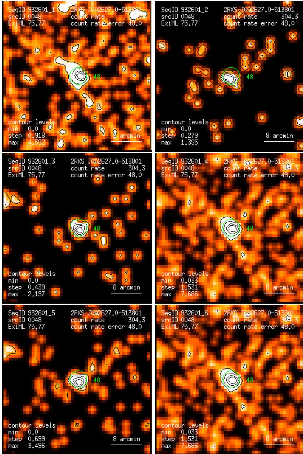
Figure 48: RASS 932601: detection 0048: band rate images, Gaussian filter: (1) PSPC channels 11 – 41, (2) 52 – 90, (3) 91 – 201, (4) 11 – 235, (5) 52 – 201, (6) 11 – 201. Broad band rates in counts/ks. Band rate contour levels in counts/ks/arcmin 2 .
