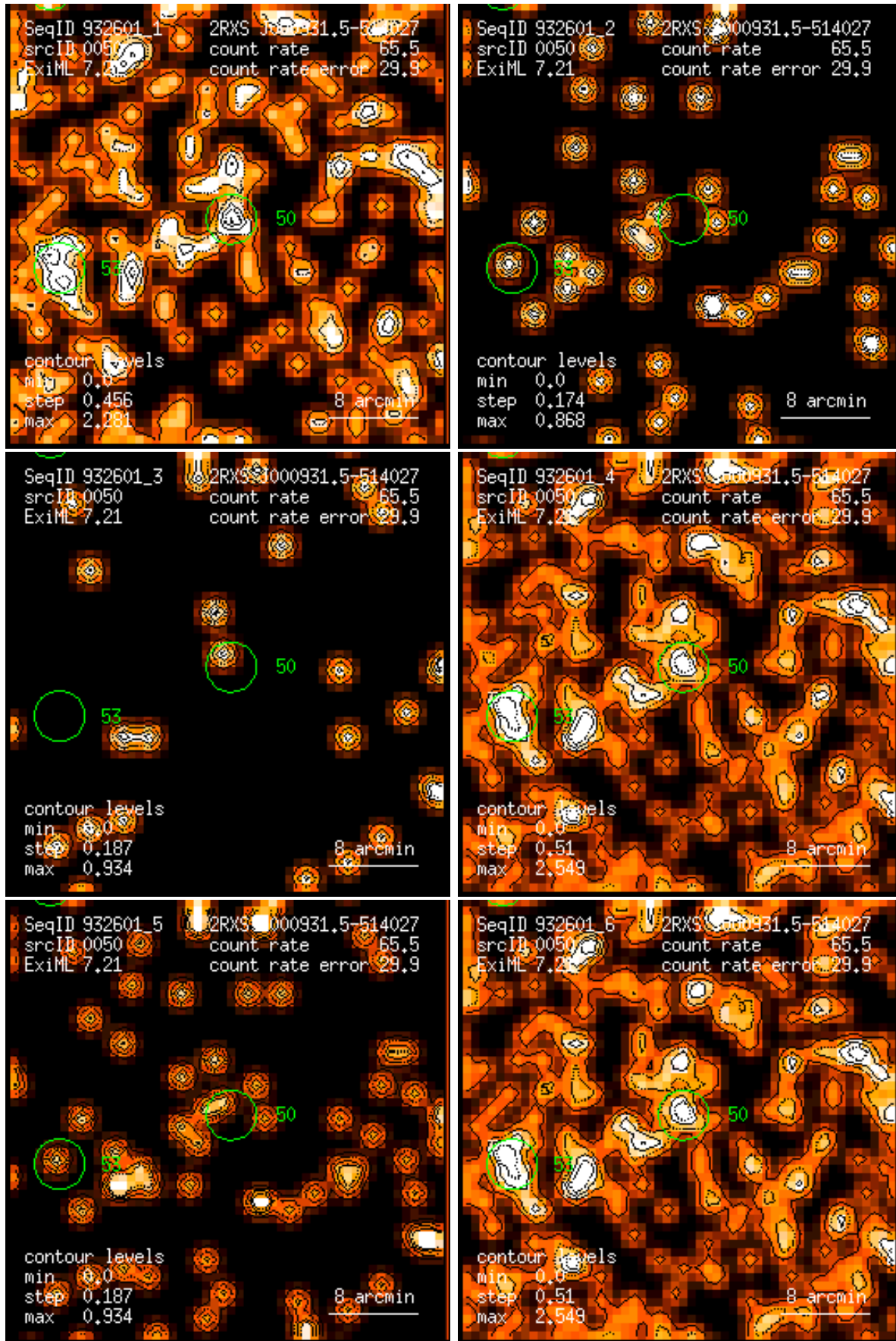
Figure 50: RASS 932601: detection 0050: band rate images, Gaussian filter: (1) PSPC channels 11 – 41, (2) 52 – 90, (3) 91 – 201, (4) 11 – 235, (5) 52 – 201, (6) 11 – 201. Broad band rates in counts/ks. Band rate contour levels in counts/ks/arcmin 2 .
