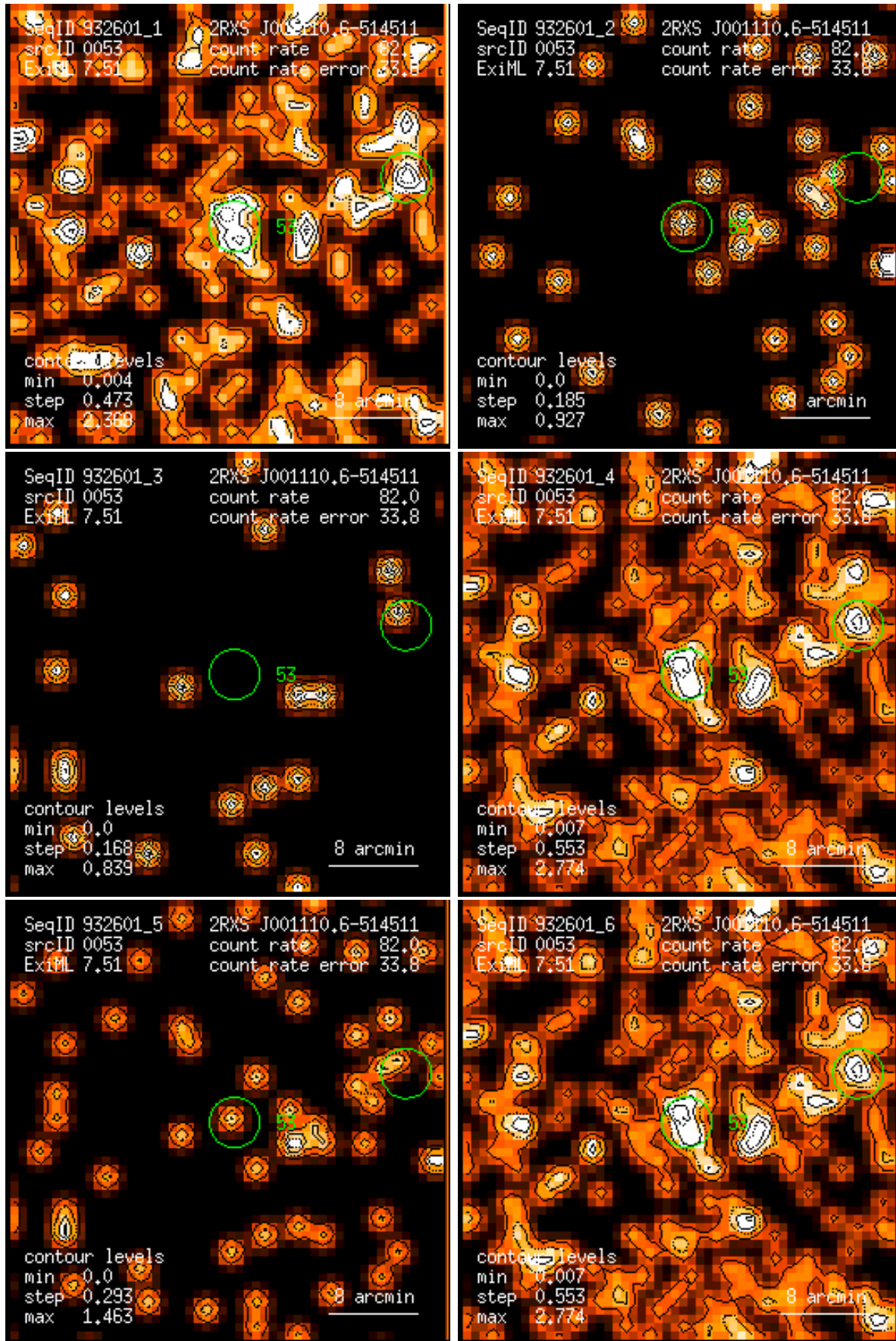
Figure 53: RASS 932601: detection 0053: band rate images, Gaussian filter: (1) PSPC channels 11 – 41, (2) 52 – 90, (3) 91 – 201, (4) 11 – 235, (5) 52 – 201, (6) 11 – 201. Broad band rates in counts/ks. Band rate contour levels in counts/ks/arcmin 2 .
