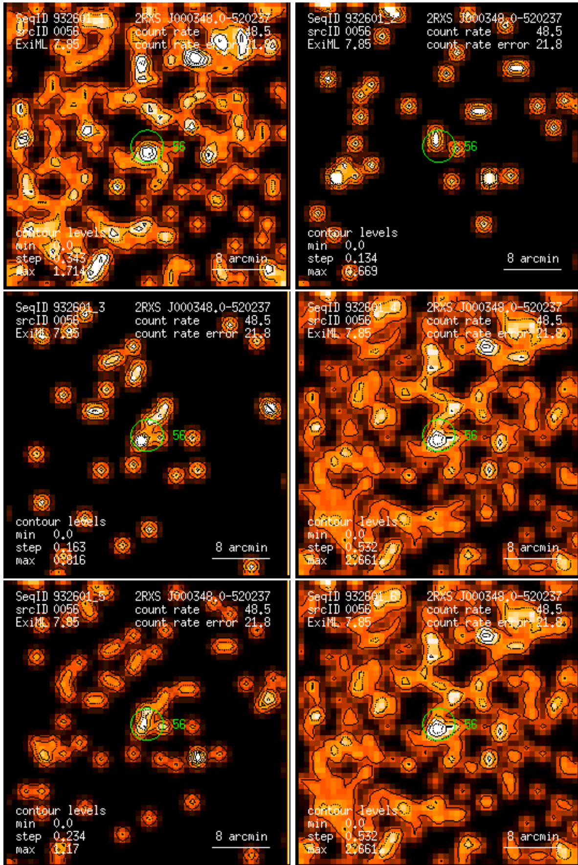
Figure 56: RASS 932601: detection 0056: band rate images, Gaussian filter: (1) PSPC channels 11 – 41, (2) 52 – 90, (3) 91 – 201, (4) 11 – 235, (5) 52 – 201, (6) 11 – 201. Broad band rates in counts/ks. Band rate contour levels in counts/ks/arcmin 2 .
