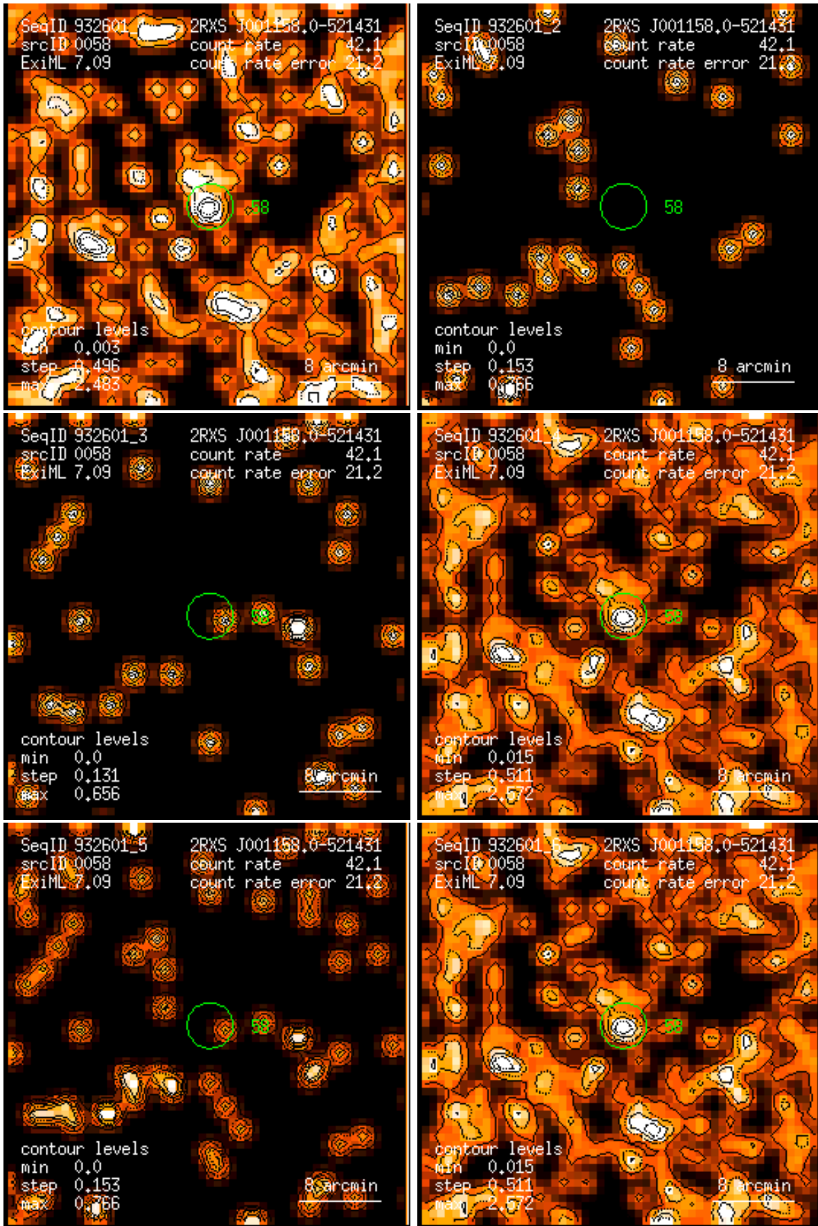
Figure 58: RASS 932601: detection 0058: band rate images, Gaussian filter: (1) PSPC channels 11 – 41, (2) 52 – 90, (3) 91 – 201, (4) 11 – 235, (5) 52 – 201, (6) 11 – 201. Broad band rates in counts/ks. Band rate contour levels in counts/ks/arcmin 2 .
