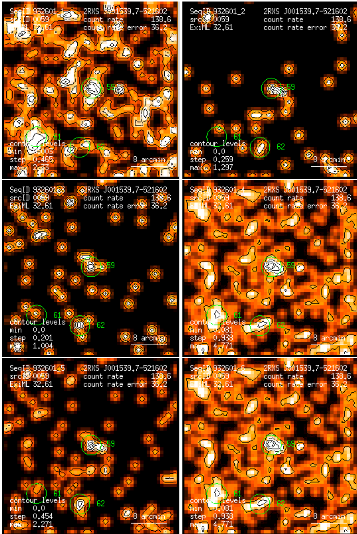
Figure 59: RASS 932601: detection 0059: band rate images, Gaussian filter: (1) PSPC channels 11 – 41, (2) 52 – 90, (3) 91 – 201, (4) 11 – 235, (5) 52 – 201, (6) 11 – 201. Broad band rates in counts/ks. Band rate contour levels in counts/ks/arcmin 2 .
